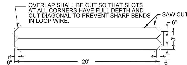
TYPICAL "TYPE F" MODIFIED BICYCLE INDUCTIVE LOOP
