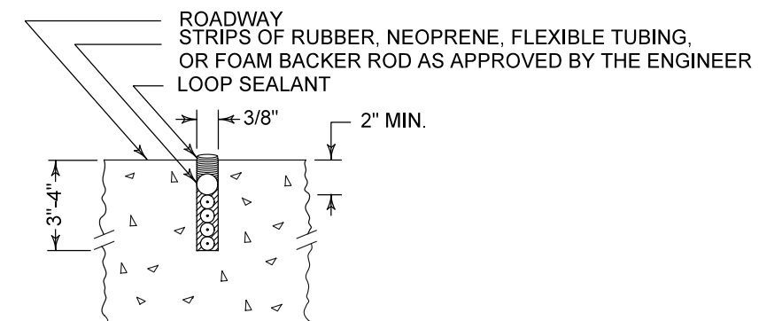
LOOP SECTION
