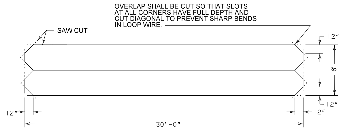
TYPICAL "TYPE F" VEHICLE INDUCTIVE LOOP
