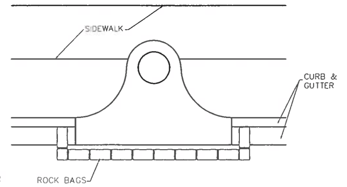
COMPLETED INLET
