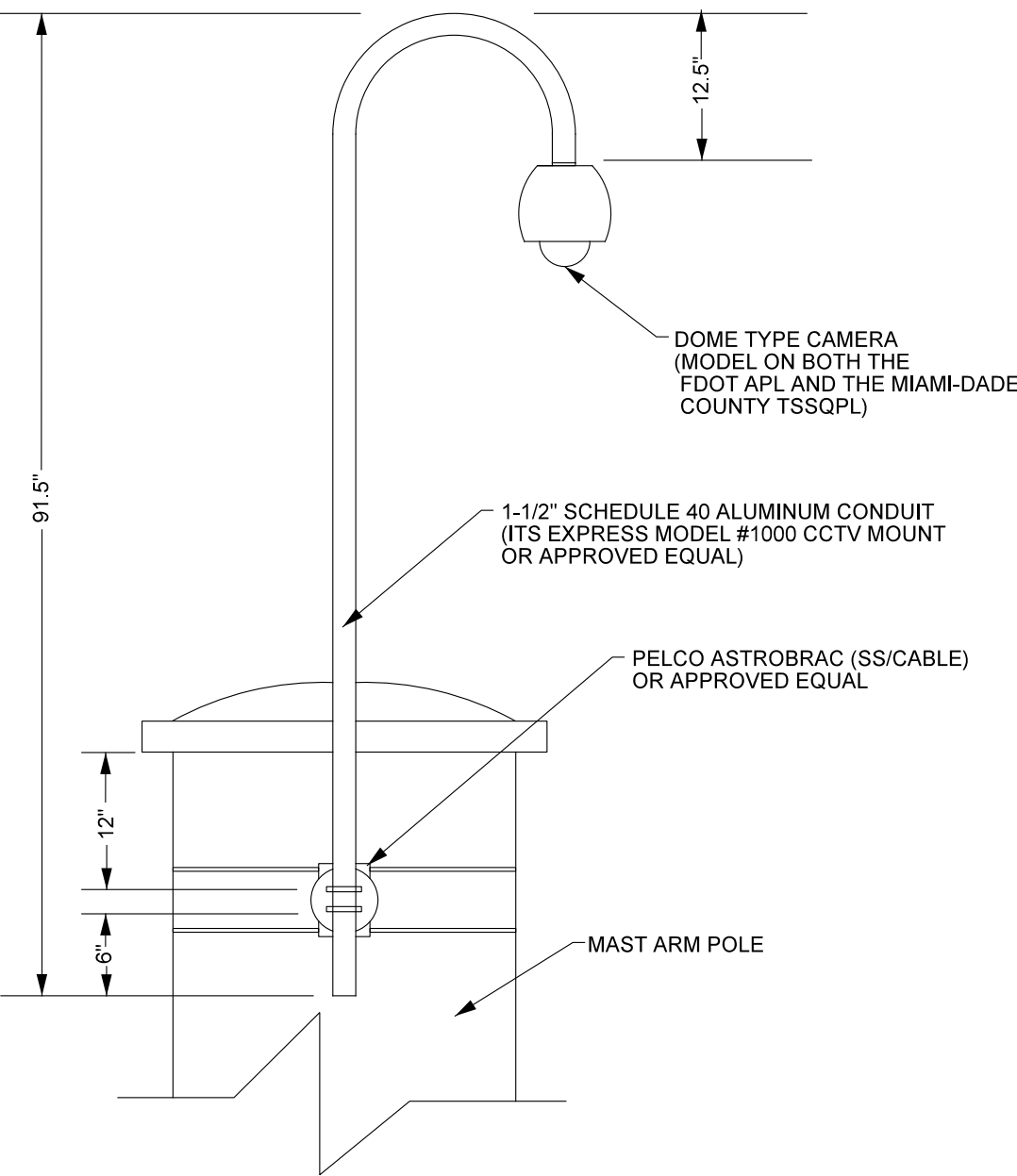
MAST ARM POLE MOUNT
