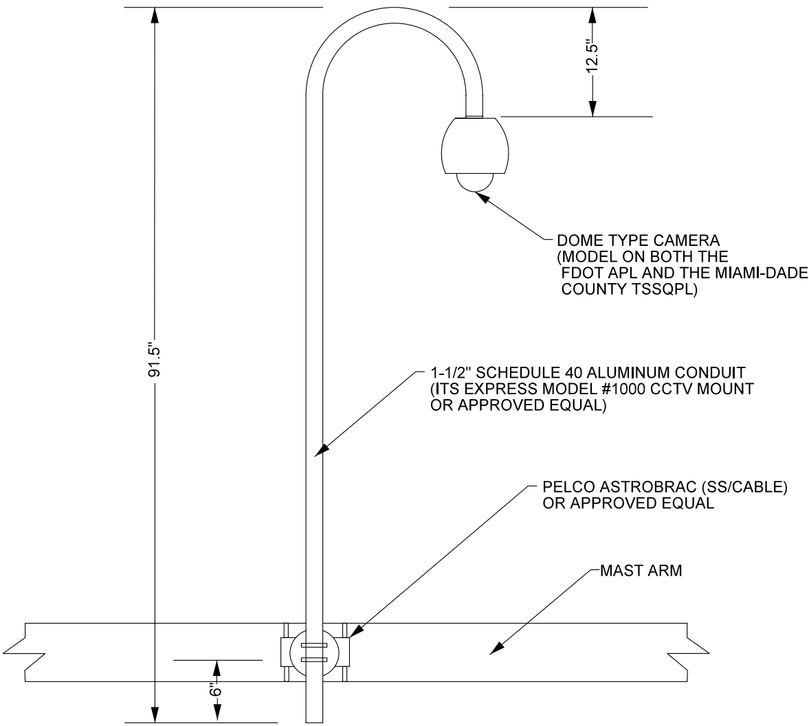
MAST ARM MOUNT
