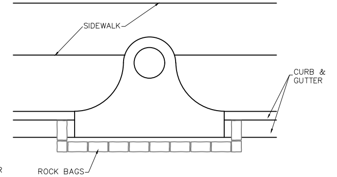
COMPLETED INLET
