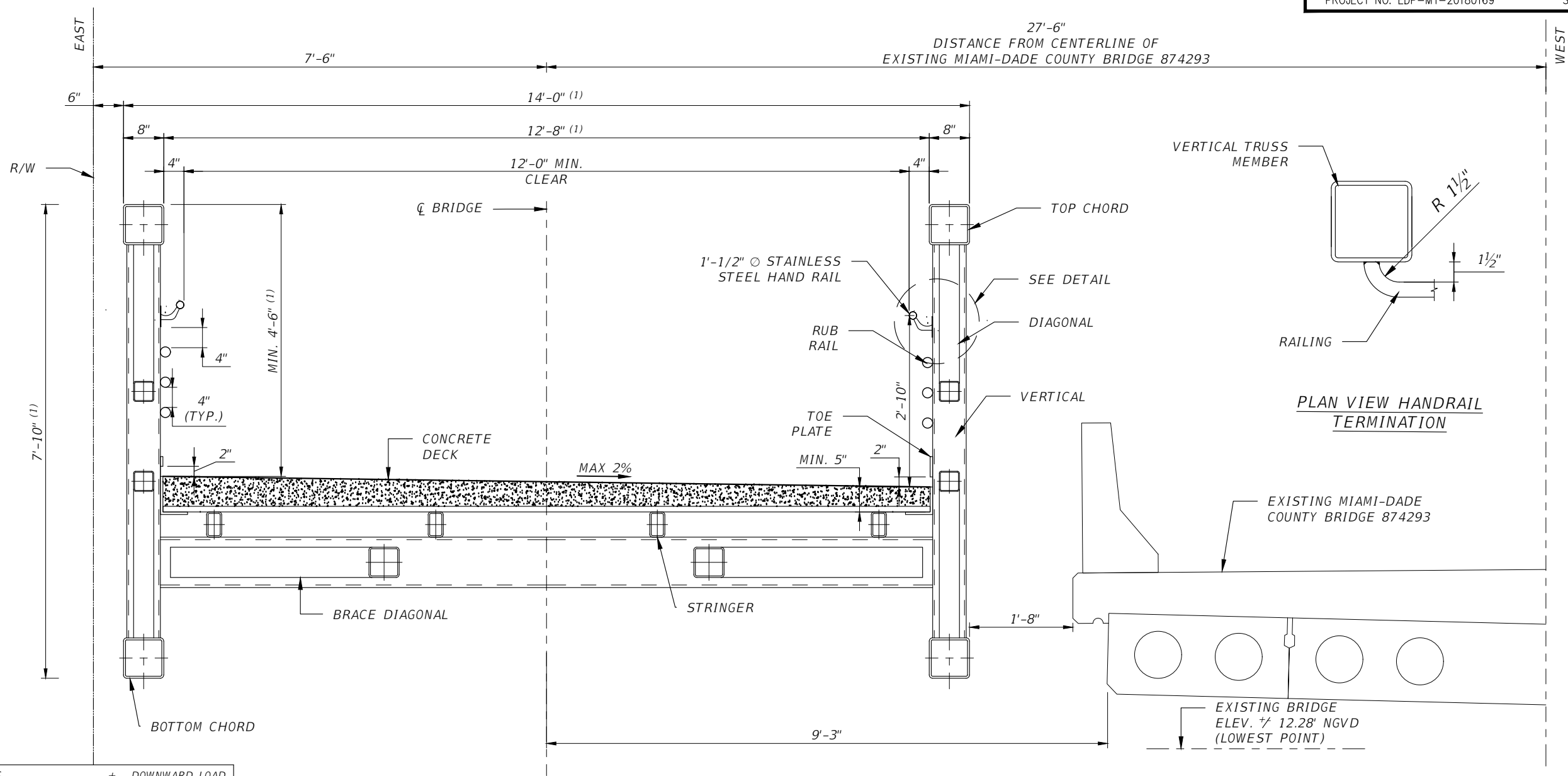
PROPOSED TYPICAL CROSS SECTION
