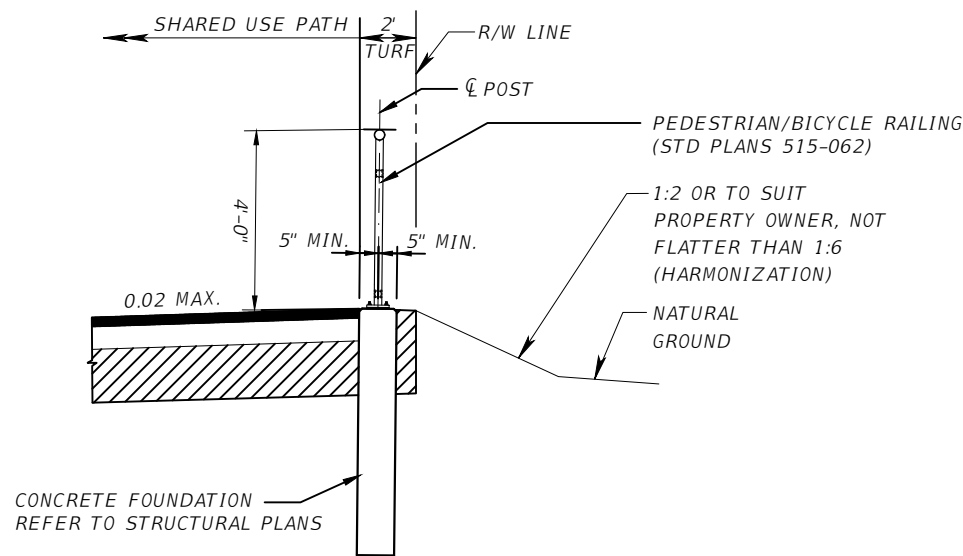
TYPICAL SECTION AT RAILING SEE ROADWAY PLAN FOR RAILING LIMITS
