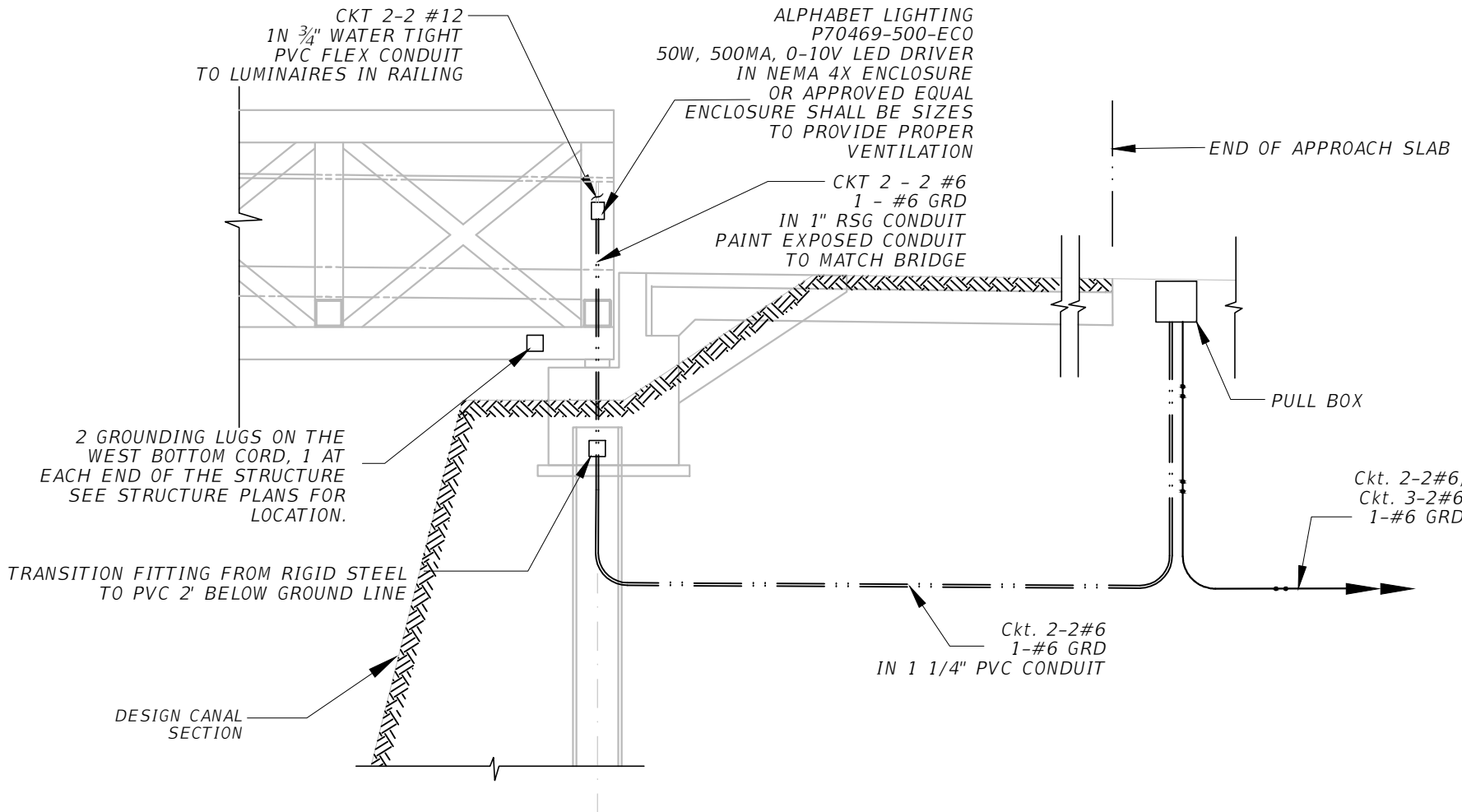
ELEVATION 1 - 1 (EAST ELEVATION SHOWN) (WEST ELEVATION SIMILAR) N.T.S.
