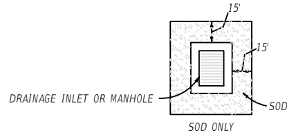
INLET SODDING NTS
