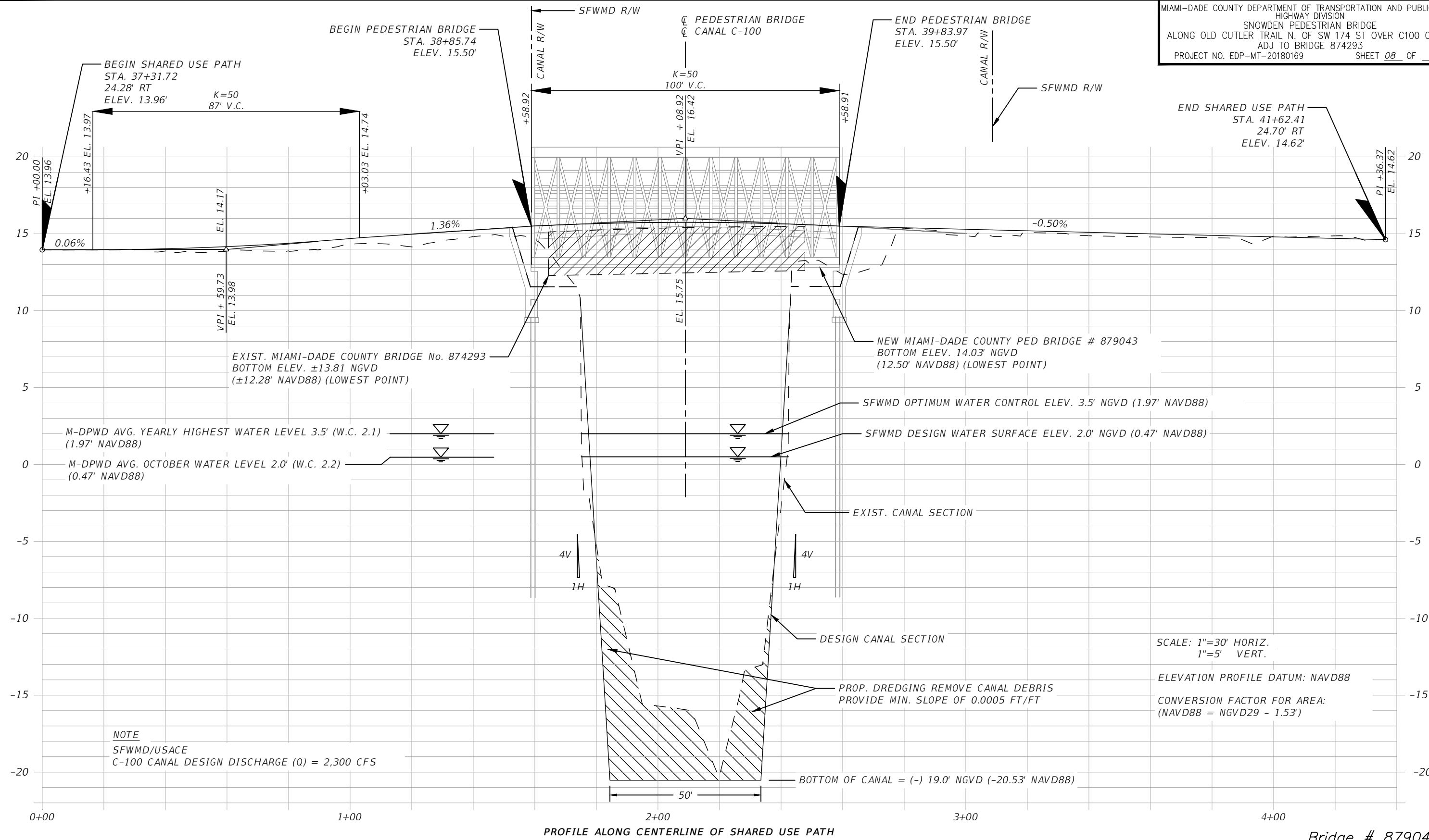
Bridge # 879043
