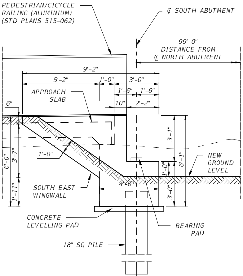
EAST SECTION VIEW
