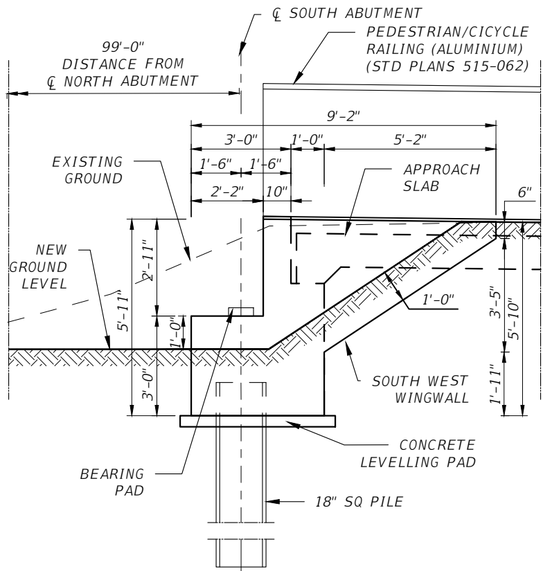
WEST SECTION VIEW
