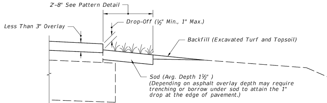
SHOULDER TREATMENT 1 (STD PLANS 570-010) STA. 37+31.72 TO STA. 38+85.74 STA. 39+89.97 + STA. 41+62.41
