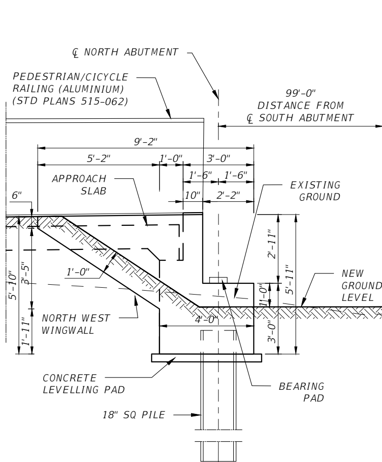
EAST SECTION VIEW
