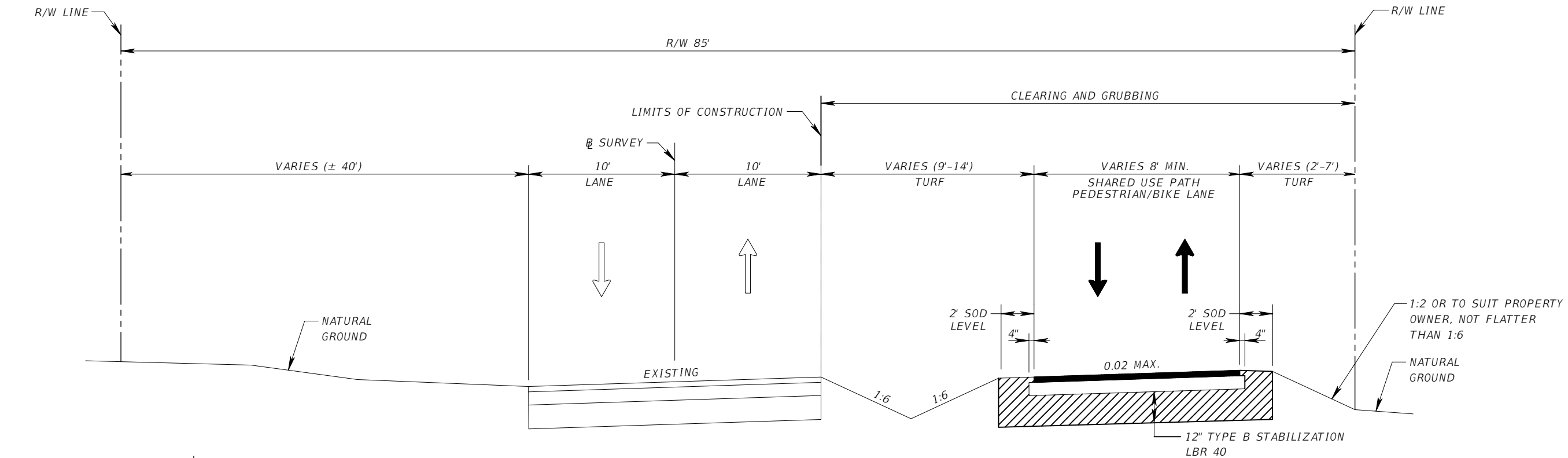
TYPICAL SECTION OLD CUTLER RD STA. 37+31.72 TO STA. 38+85.86
