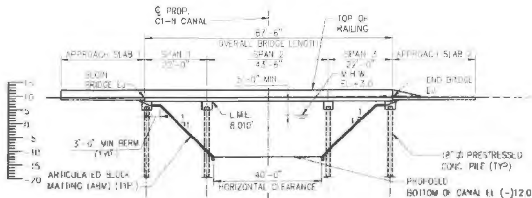
PROPOSED BRIDGE SECTION
