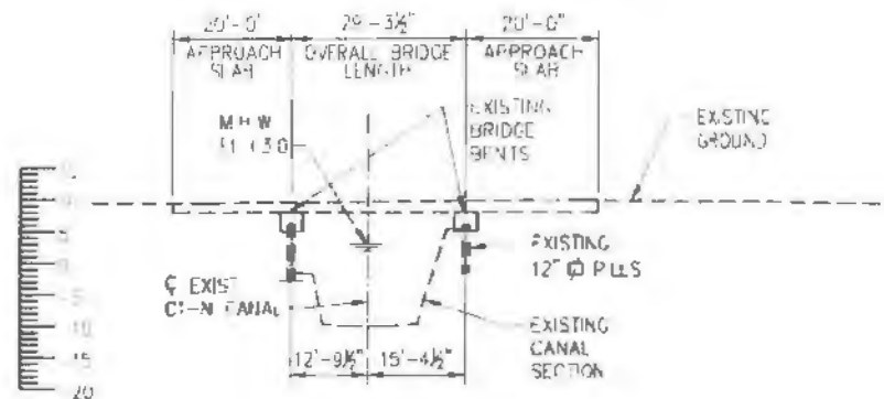
EXISTING BRIDGE SECTION
