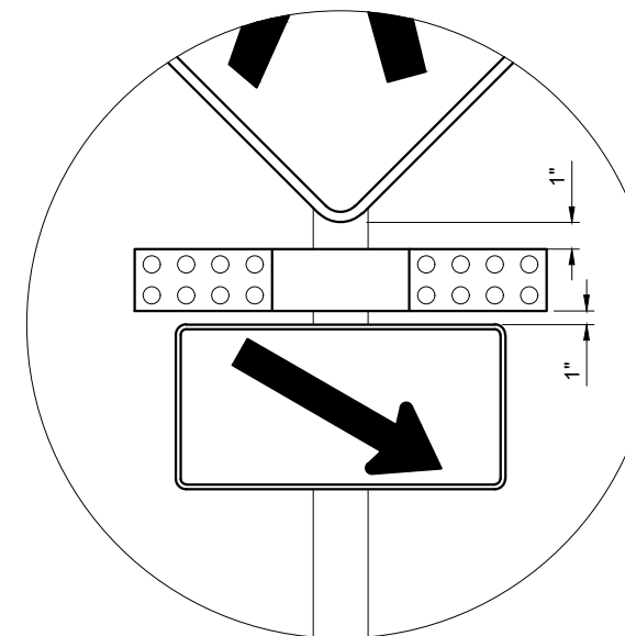
DETAIL A
