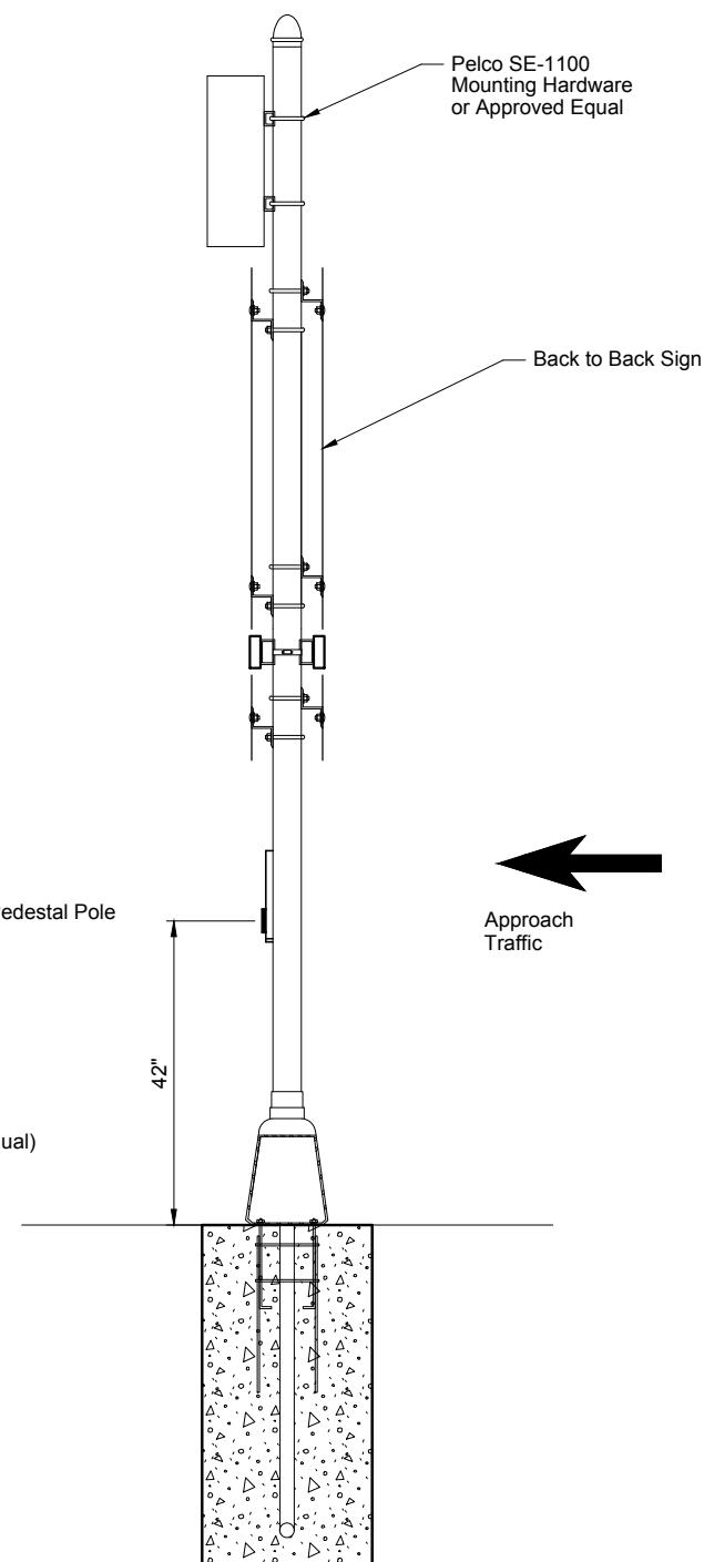
AC POWERED RRFB SIDE VIEW
