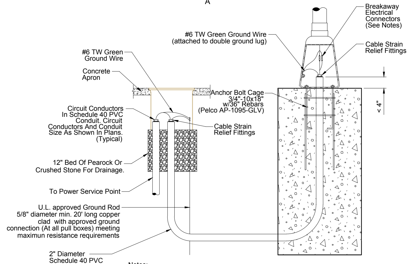
DETAIL A
