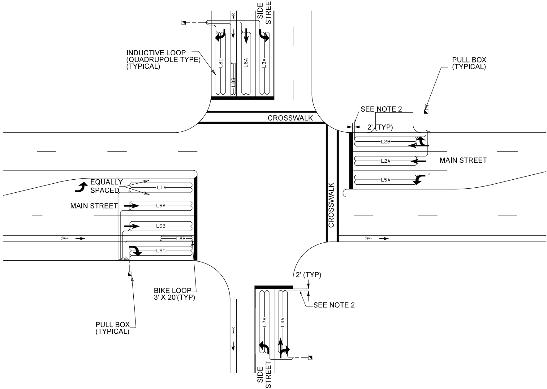
TYPICAL INDUCTIVE LOOP PLACEMENT NOT TO SCALE
