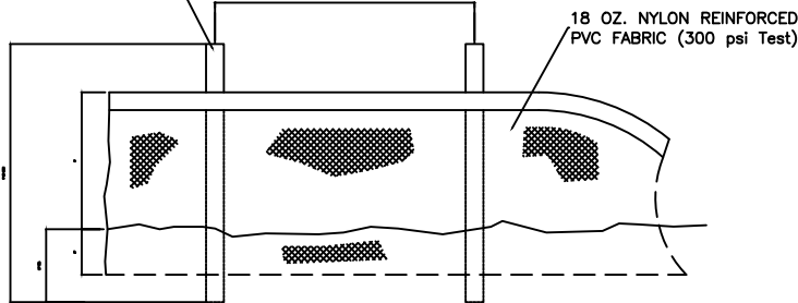
STAKED TURBIDITY BARRIER (TYP.)
