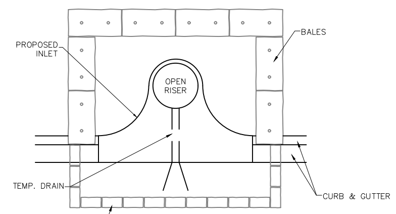
PARTIAL INLET
