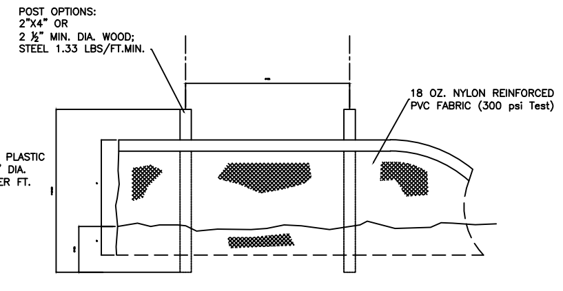
STAKED TURBIDITY BARRIER (TYP.)
