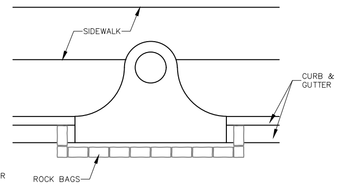
COMPLETED INLET
