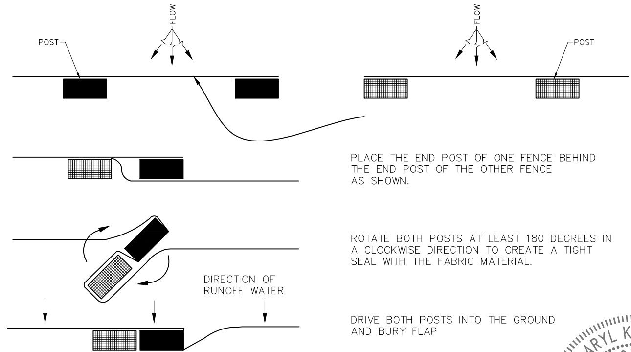
PLANT VIEW
