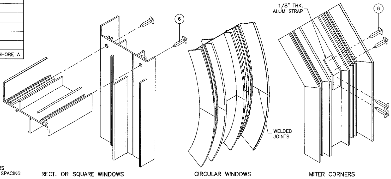
CORNER DETAILS
