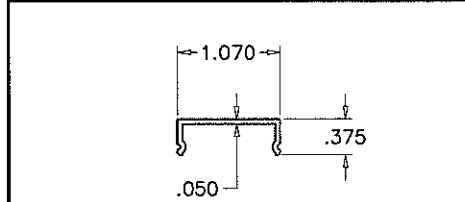
② GLAZING BEAD
