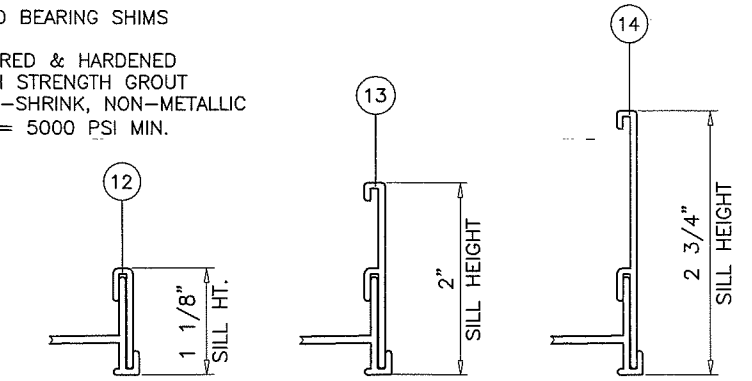
SILL HEIGHT VS WATER RESISTANCE EXT.(+) LOAD SEE SHEET 5 CHART 1 FOR DOOR CAPACITY
