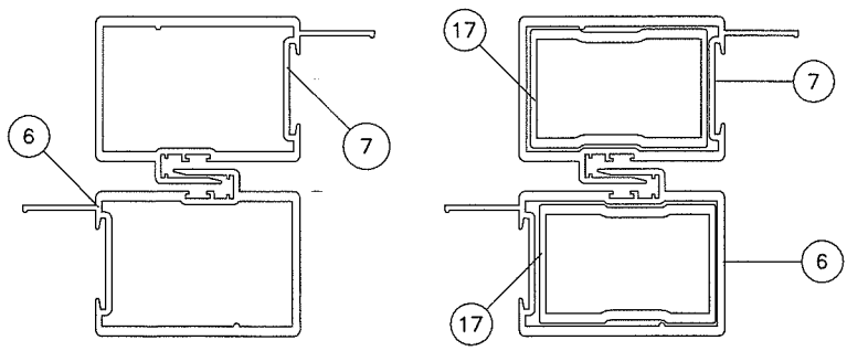
INTERLOCKS WITHOUT REINF. INTERLOCKS WITH REINF.
