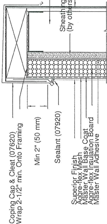
Cap Detail
