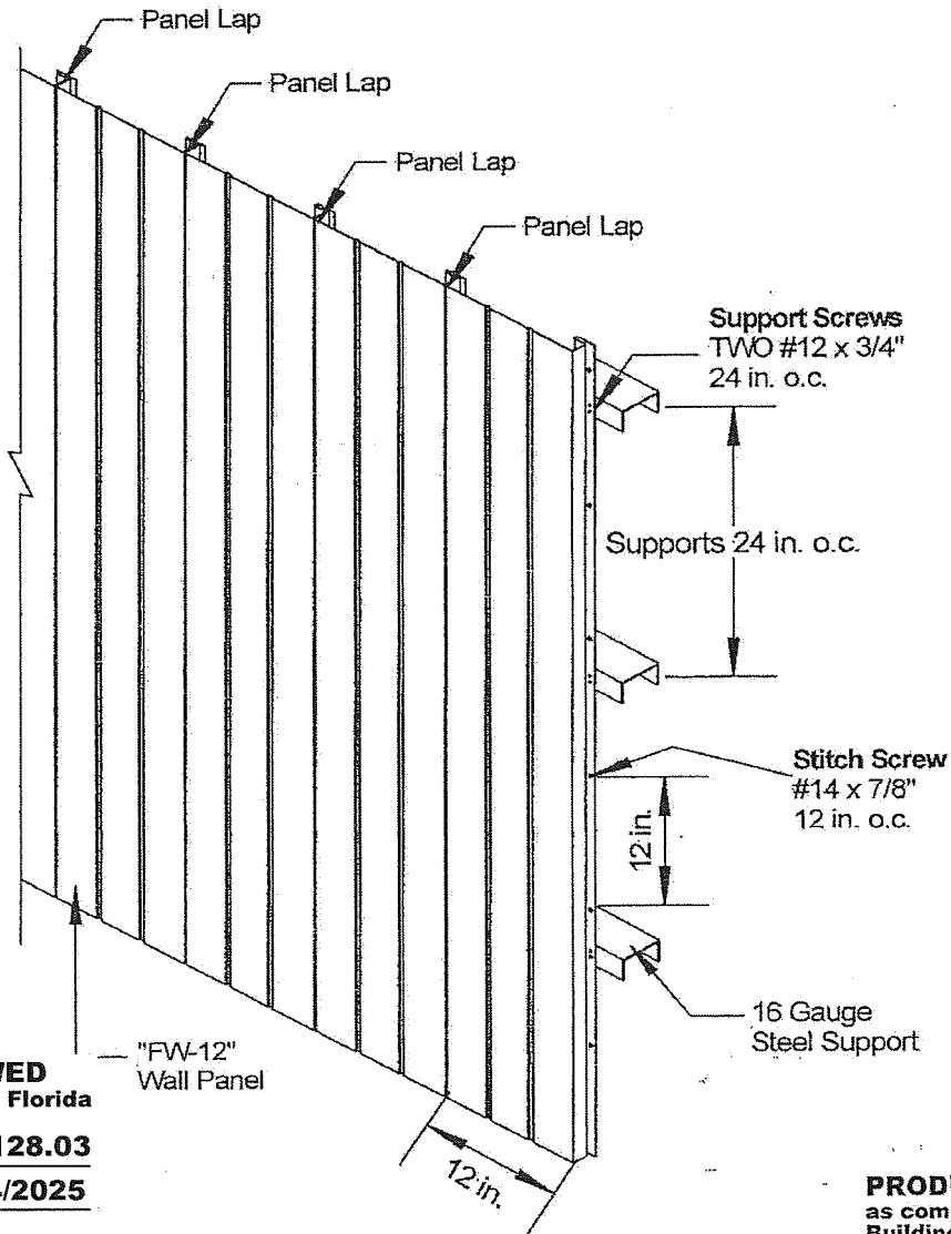
TYPICAL ELEVATION VIEW OUTSIDE OF WALL ASSEMBLY
