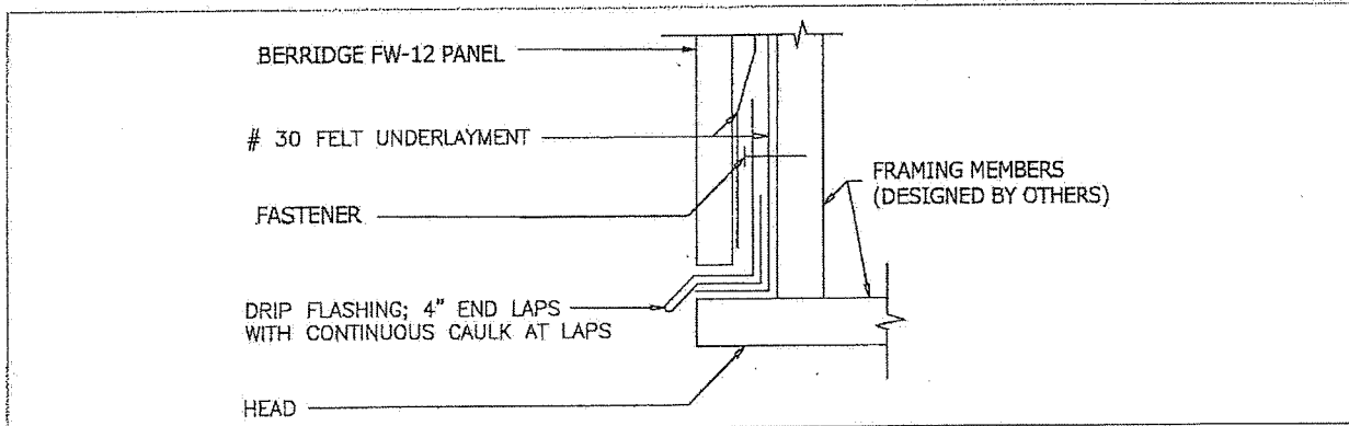
TYPICAL HEADER DETAIL
