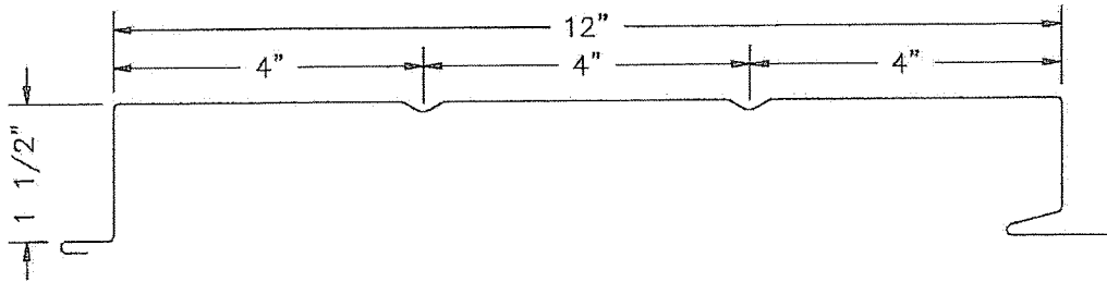
TYPICAL PANEL PROFILE
