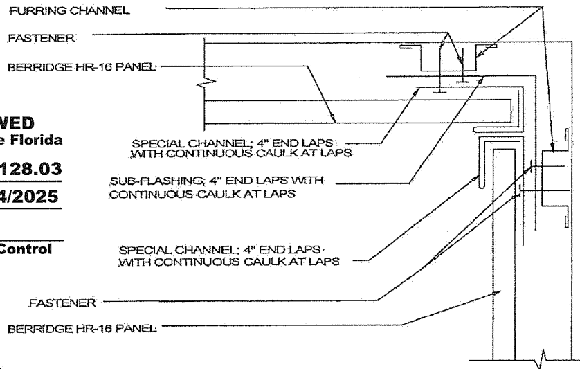
TYPICAL INSIDE CORNER DETAIL
