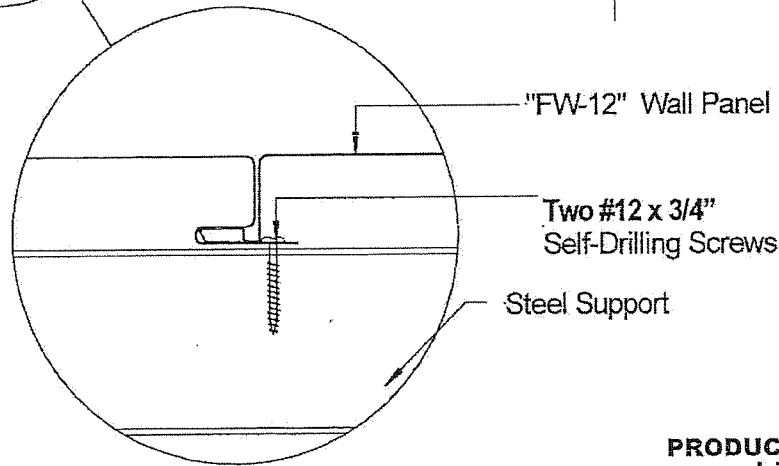
TYPICAL PANEL ASSEMBLY SECTION VIEW
