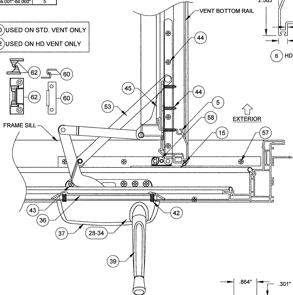
HORIZONTAL HARDWARE SECTION
