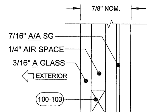
GLASS TYPE 15
