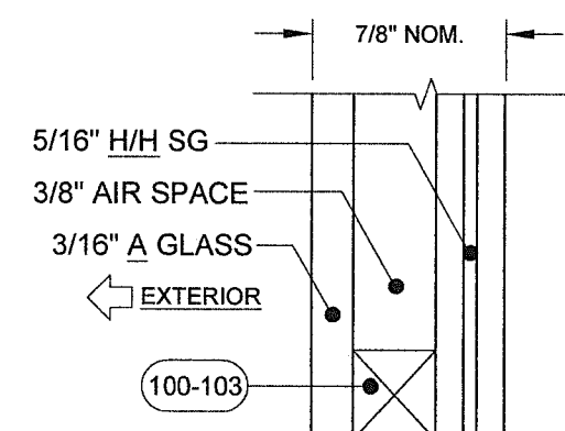
GLASS TYPE 11
