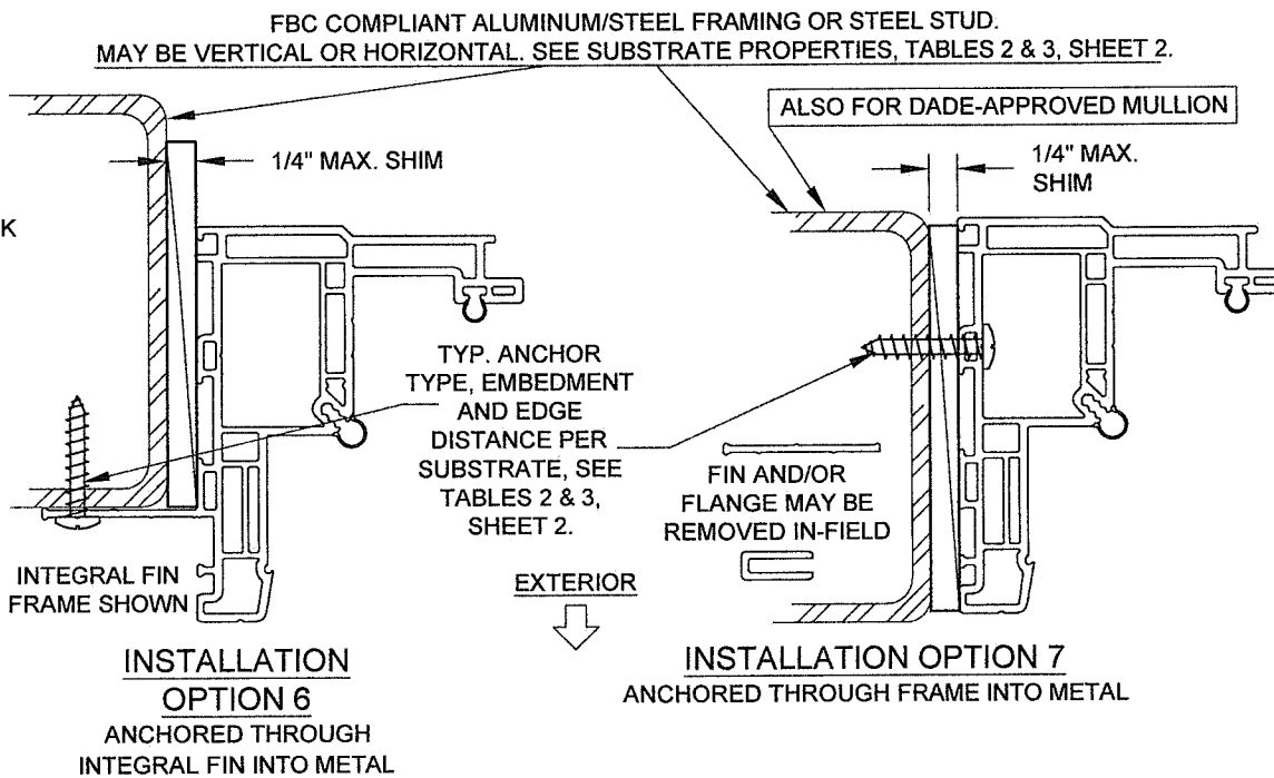
HORIZONTAL SECTION C-C
