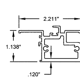
⑰ STD MEETING RAIL
