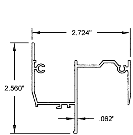
① HEAD, FLANGE FRAME
