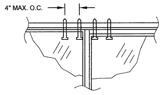
4-ANCHOR CLUSTER DETAIL
