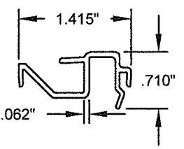
⑱ SILL TRACK
