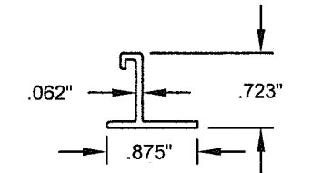
⑫ WINDLOAD ADAPTER
