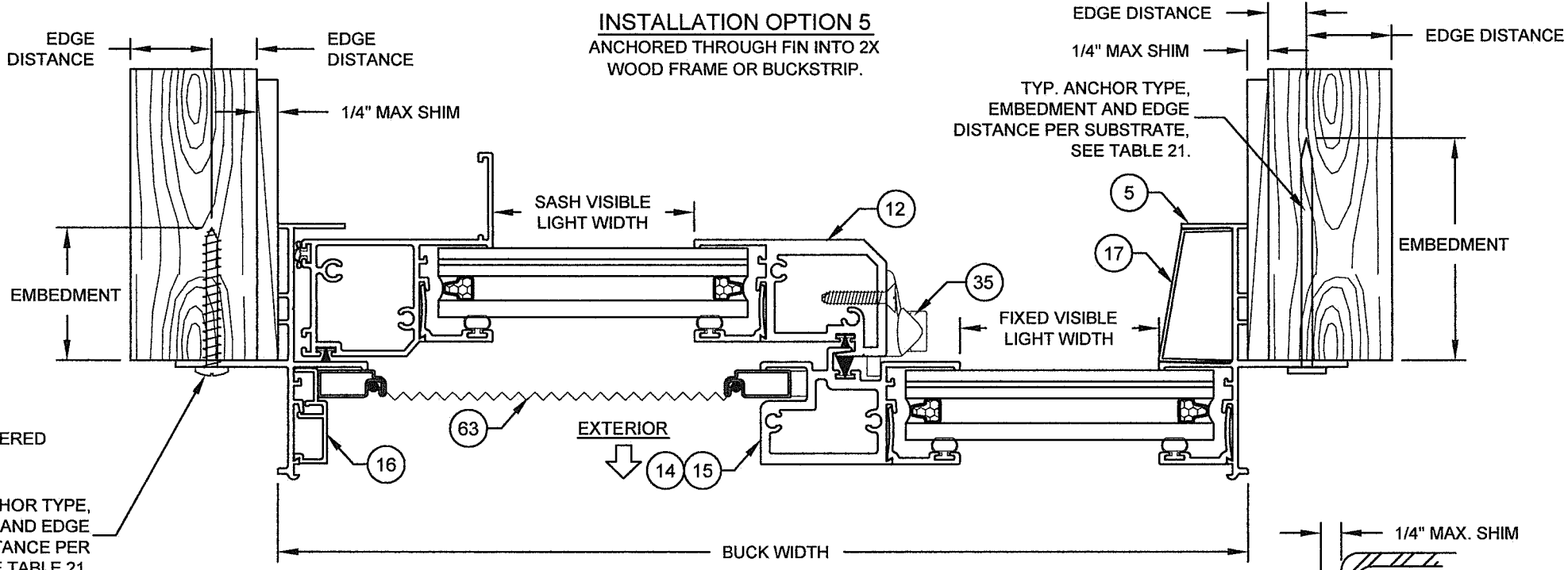
HORIZONTAL SECTION A-A (SHOWN WITH I.G. GLAZING)
