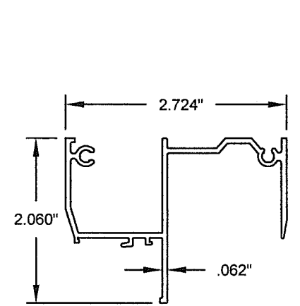
③ HEAD, EQUAL LEG FRAME
