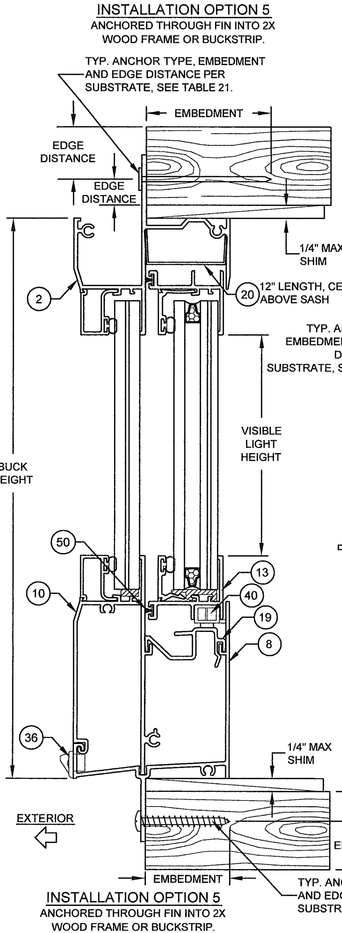
VERTICAL SECTION B-B
