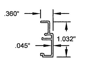
⑳ SCREEN ADAPTER
