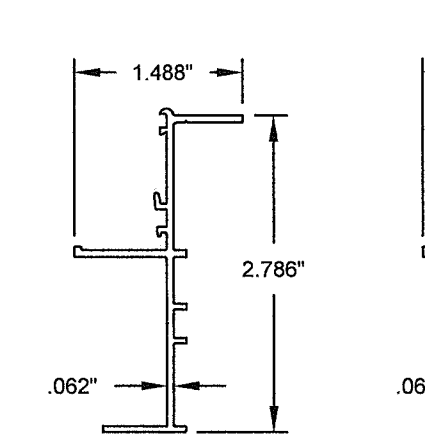
④ JAMB, FLANGE FRAME
