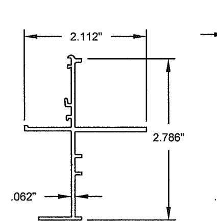
⑤ JAMB, INTEGRAL FIN FRAME
