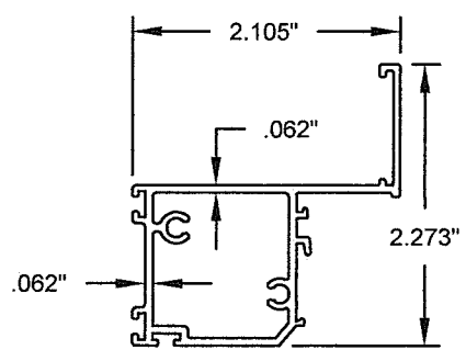
⑬ SASH PULL RAIL
