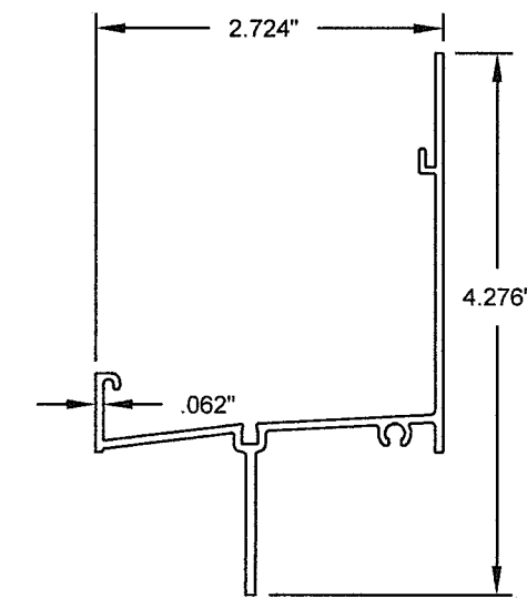
⑧ SILL, INTEGRAL FIN FRAME
