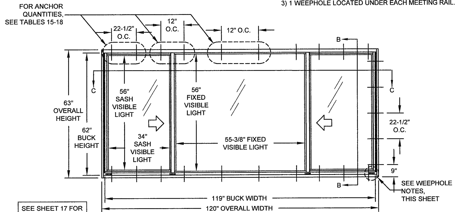
TYP. FLANGE XOX ELEVATION MAX. DIMENSIONS ALLOWED SHOWN
