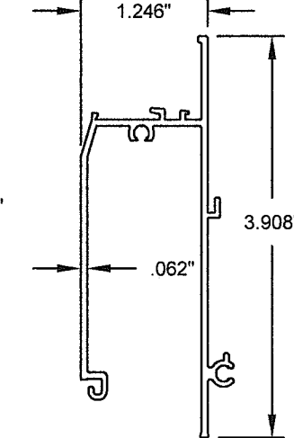
⑩ SILL ADAPTER
