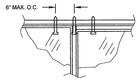
3-ANCHOR CLUSTER DETAIL
