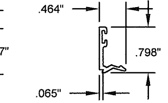
㉒ IG SNAP BEAD
