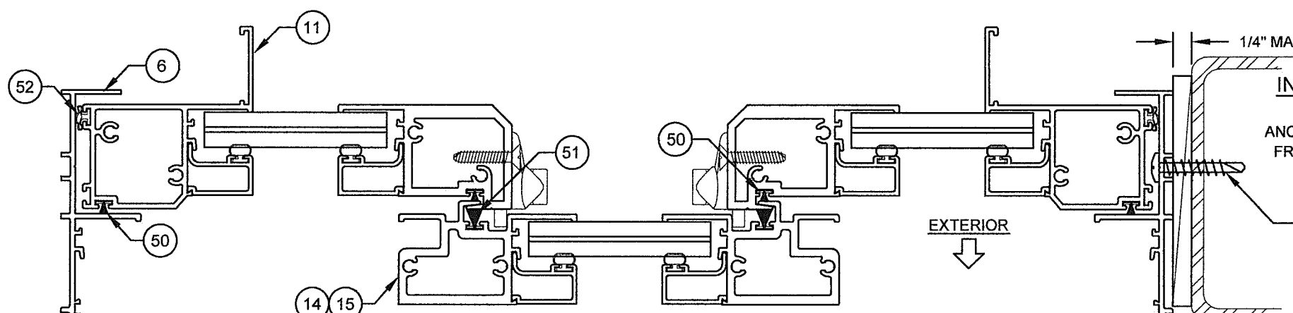
HORIZONTAL SECTION A-A (SHOWN WITH I.G. GLAZING)
