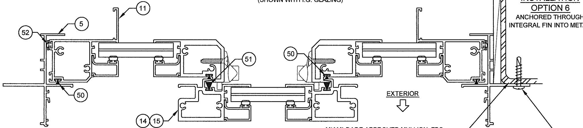
HORIZONTAL SECTION A-A (SHOWN WITH I.G. GLAZING)
