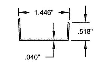
⑲ ANTI-LIFT CLIP
