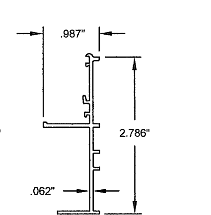
⑥ JAMB, EQUAL LEG FRAME
