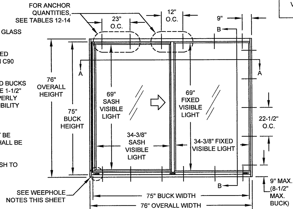
TYP. FLANGE XO ELEVATION (OX SIM.) MAX. DIMENSIONS ALLOWED SHOWN
