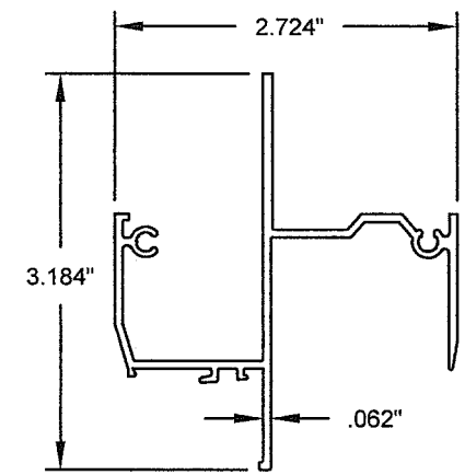
② HEAD, INTEGRAL FIN FRAME
