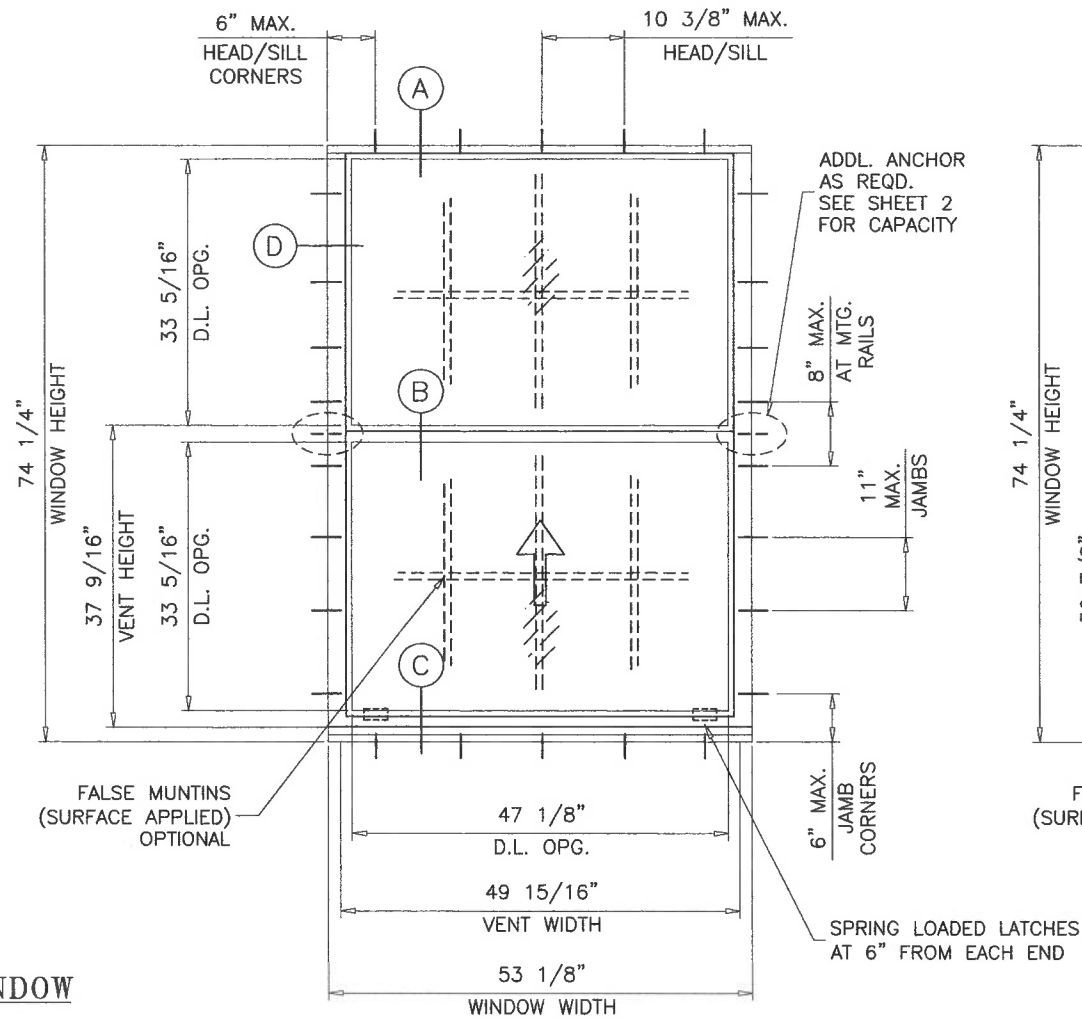
TYPICAL ELEVATION
