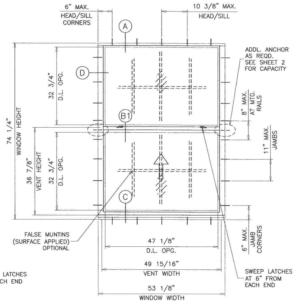
TYPICAL ELEVATION
