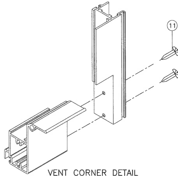
VENT CORNER DETAIL
