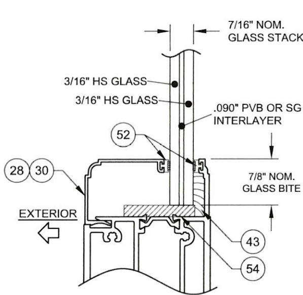
GLASS TYPE 1 (WITH PVB) GLASS TYPE 3 (WITH SG)
