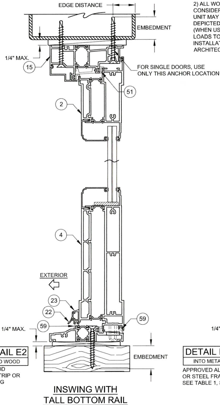
DETAIL D2 APPROVED MULLION, ALUMINUM OR STEEL FRAMING. INTO METAL
