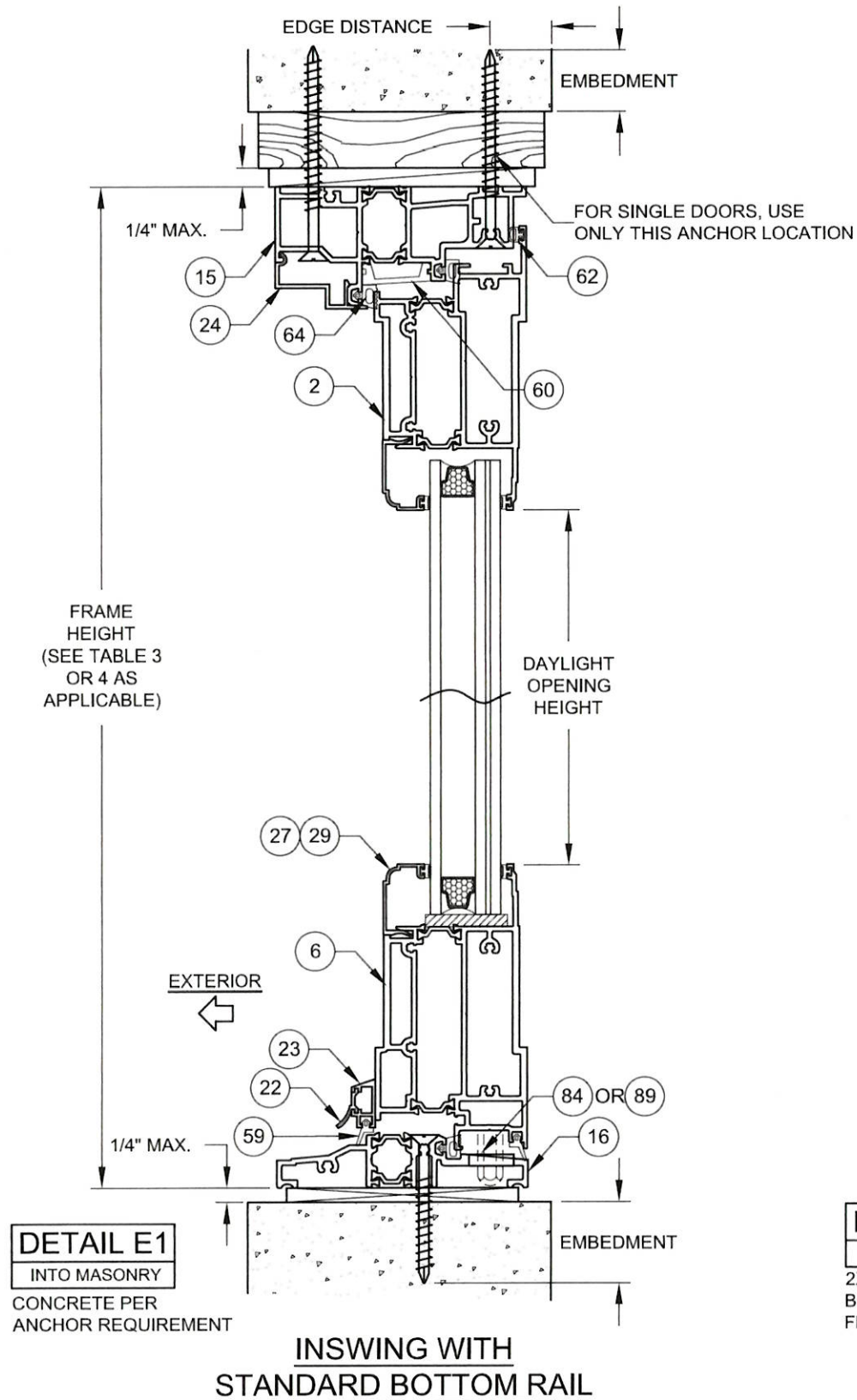
DETAIL D1 1X WOOD BUCKSTRIP. THRU 1X WOOD INTO MASONRY CONCRETE PER ANCHOR REQUIREMENT
