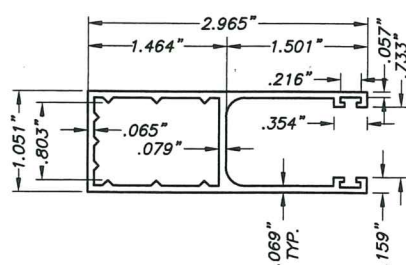
(J) TYPE 1 SIDE RAIL: 6063-T6 Alum. ALLOY SCALE: 1/2" = 1"
