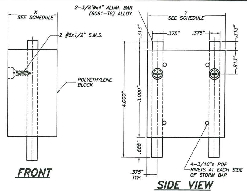
BOTTOM SPRING-LOADED SYSTEM SCALE: 1/2" = 1"
