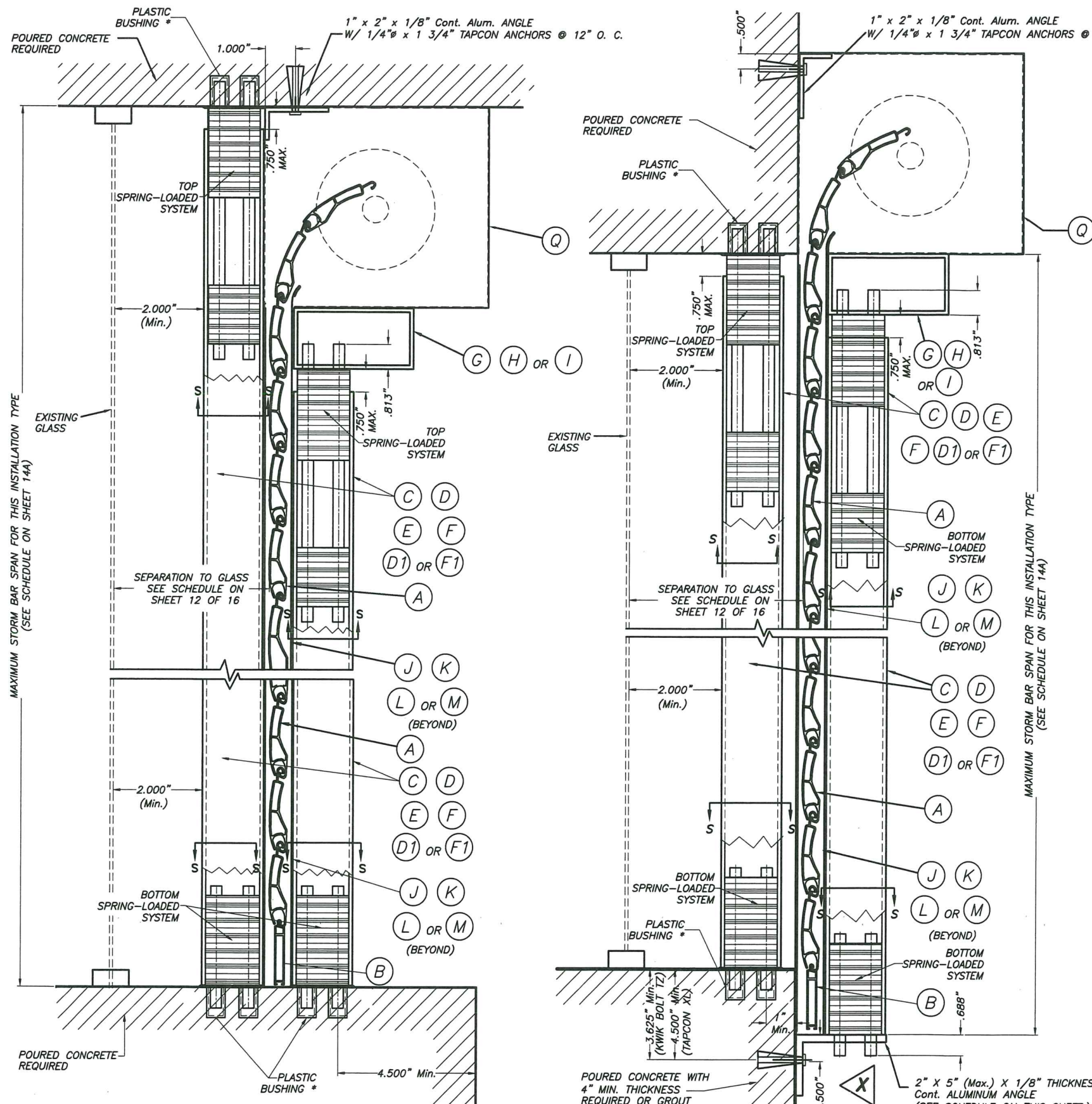
CEILING & FLOOR MOUNTING SECTION V-V(2) INSTALLATION W/ REMOVABLE STORM BARS W/SPRING-LOADED SYSTEM *
