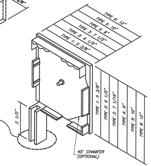
(R) BOX SIDE BRACKET TYPES
