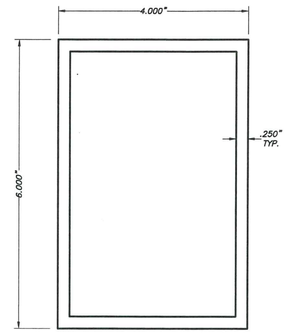
(P) TYPE 3 MULLION: 6" EXTRUDED MULLION 6063-T6 ALUMINUM ALLOY SCALE: 1/2" = 1"
