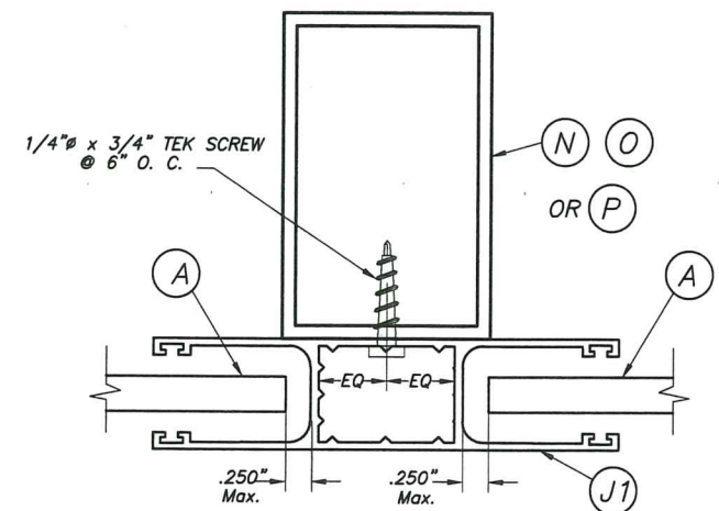
SECTION R - R (2) : MULLION MOUNT (FACE MOUNT)
