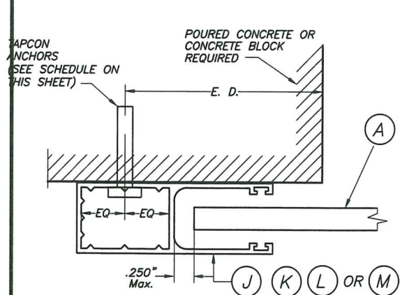
SECTION P - P (1) : WALL MOUNT
