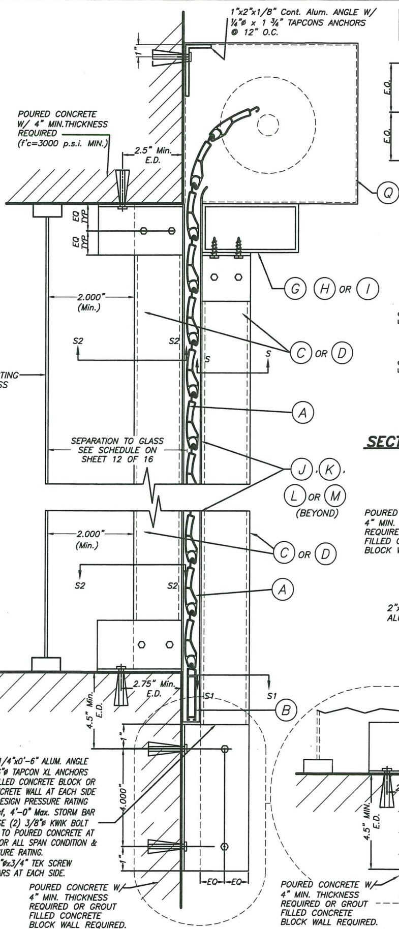
WALL MOUNTING SECTION V-V(1) INSTALLATION W/ FIXED STORM BARS W/ CONCRETE ANCHORS SCALE: 1/4" = 1"
