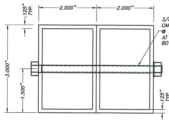
(D1) TYPE 5 STORM BAR: 3" EXTRUDED STORM BAR 6063-T6 ALUMINUM ALLOY SCALE: 1/2" = 1"
