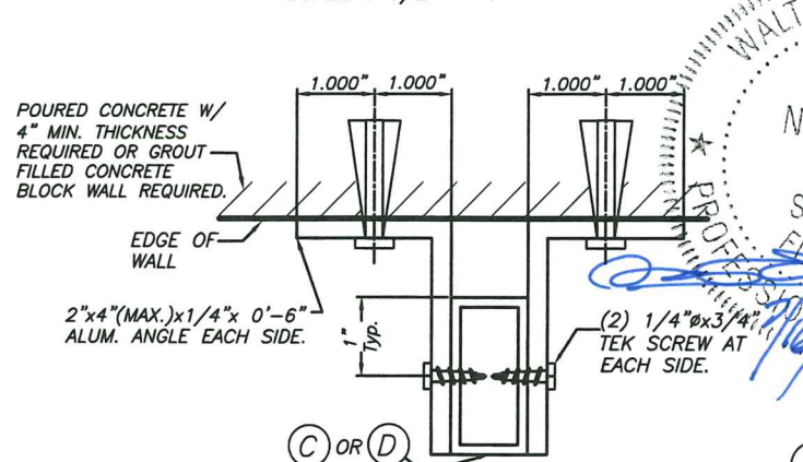
SECTION S - S (FOR REMOVABLE STORM BAR) SCALE: 1/2" = 1"
