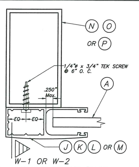
SECTION Q - Q : MULLION MOUNT (FACE MOUNT)
