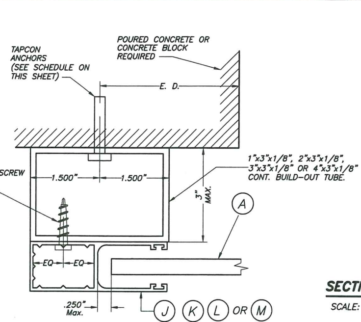
SECTION P - P (3) : BUILD-OUT MOUNT
