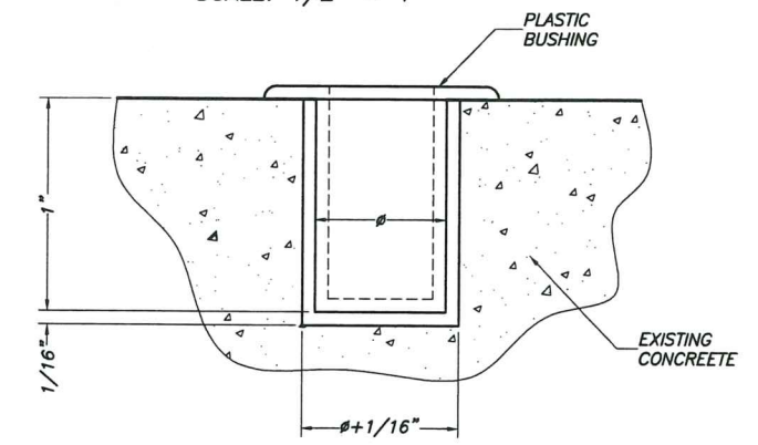
ENGAGEMENT HOLE DETAIL (IN CONCRETE) FOR REMOVABLE SPRING-LOADED STORM BARS SCALE: 1" = 1"
