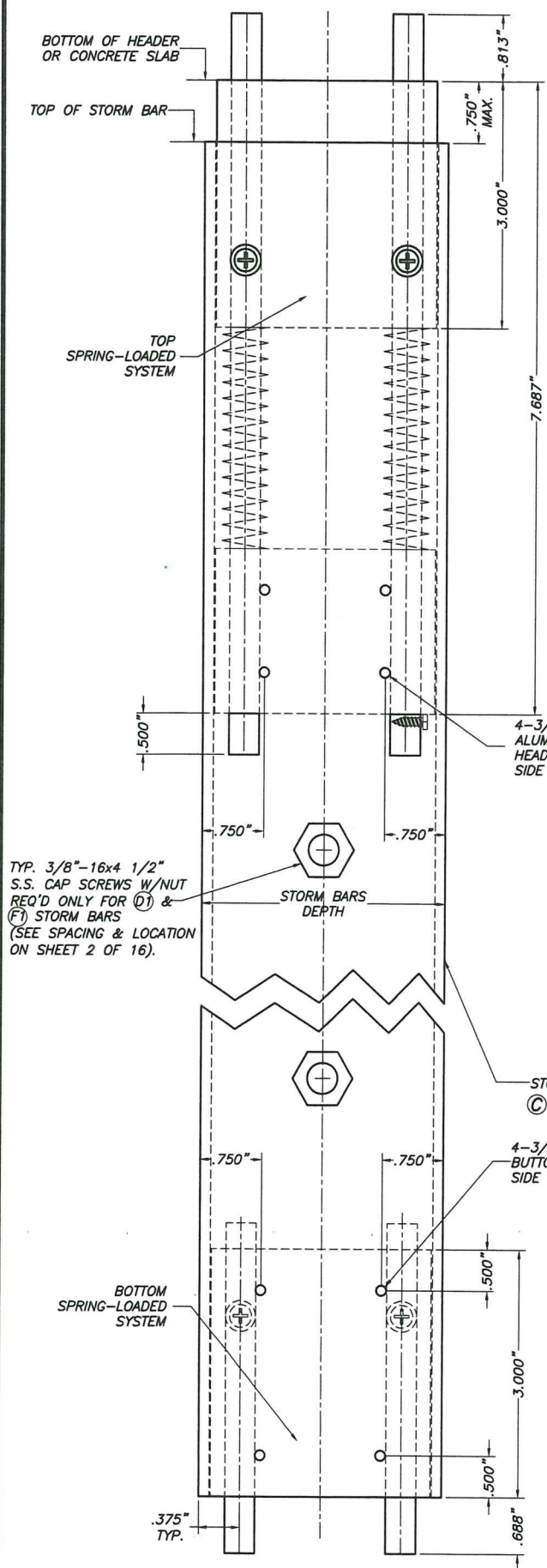
TYPICAL CONNECTION TO STORM BARS (SIDE VIEW) SCALE: 1/2" = 1"
