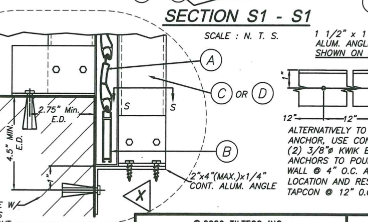
OPTIONAL STORM BAR CONNECTION
