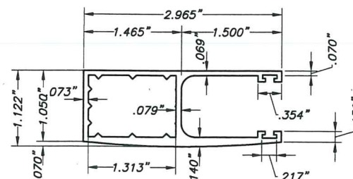
(L) TYPE 3 SIDE RAIL: 6063-T6 Alum. ALLOY SCALE: 1/2" = 1"
