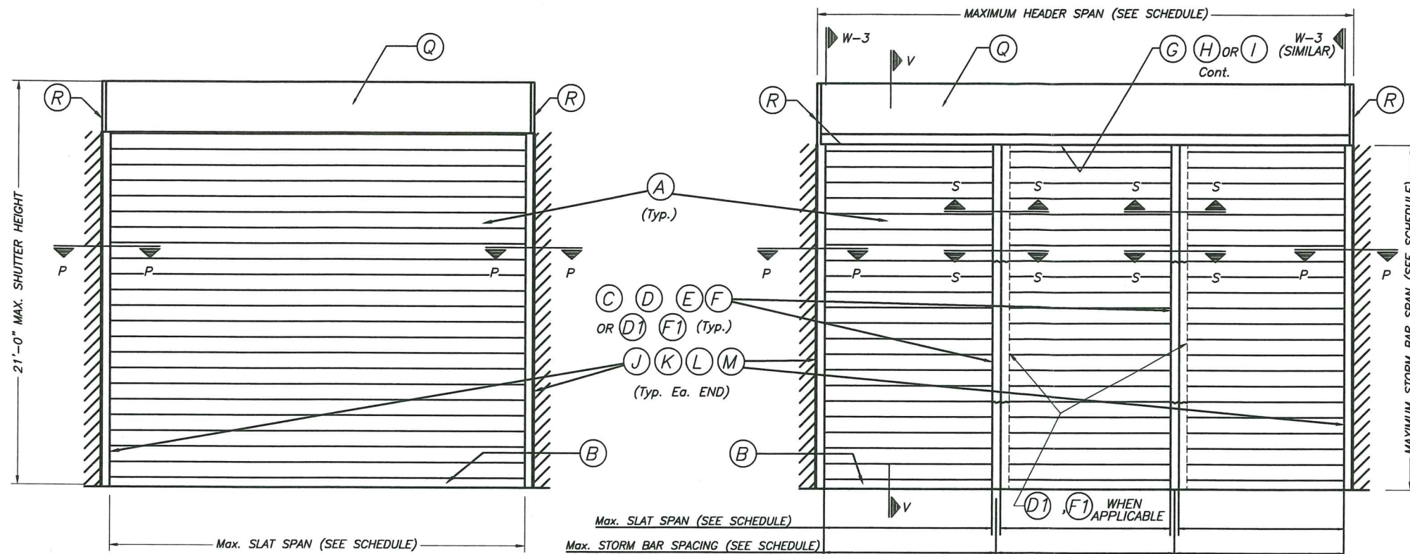
TYPICAL SINGLE UNIT ELEVATION (NO STORM BARS REQUIRED)
