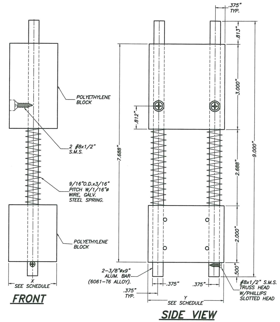
TOP SPRING-LOADED SYSTEM SCALE: 1/2" = 1"
