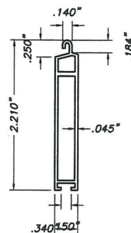
(B) TYPE 2 SLAT: EXTRUDED ALUMINUM BOTTOM SLAT 6063-T6 ALUMINUM ALLOY SCALE: 1/2" = 1"
