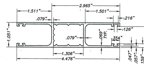
(J1) TYPE 5 SIDE RAILS: 6063-T6 Alum. ALLOY SCALE: 1/2" = 1"
