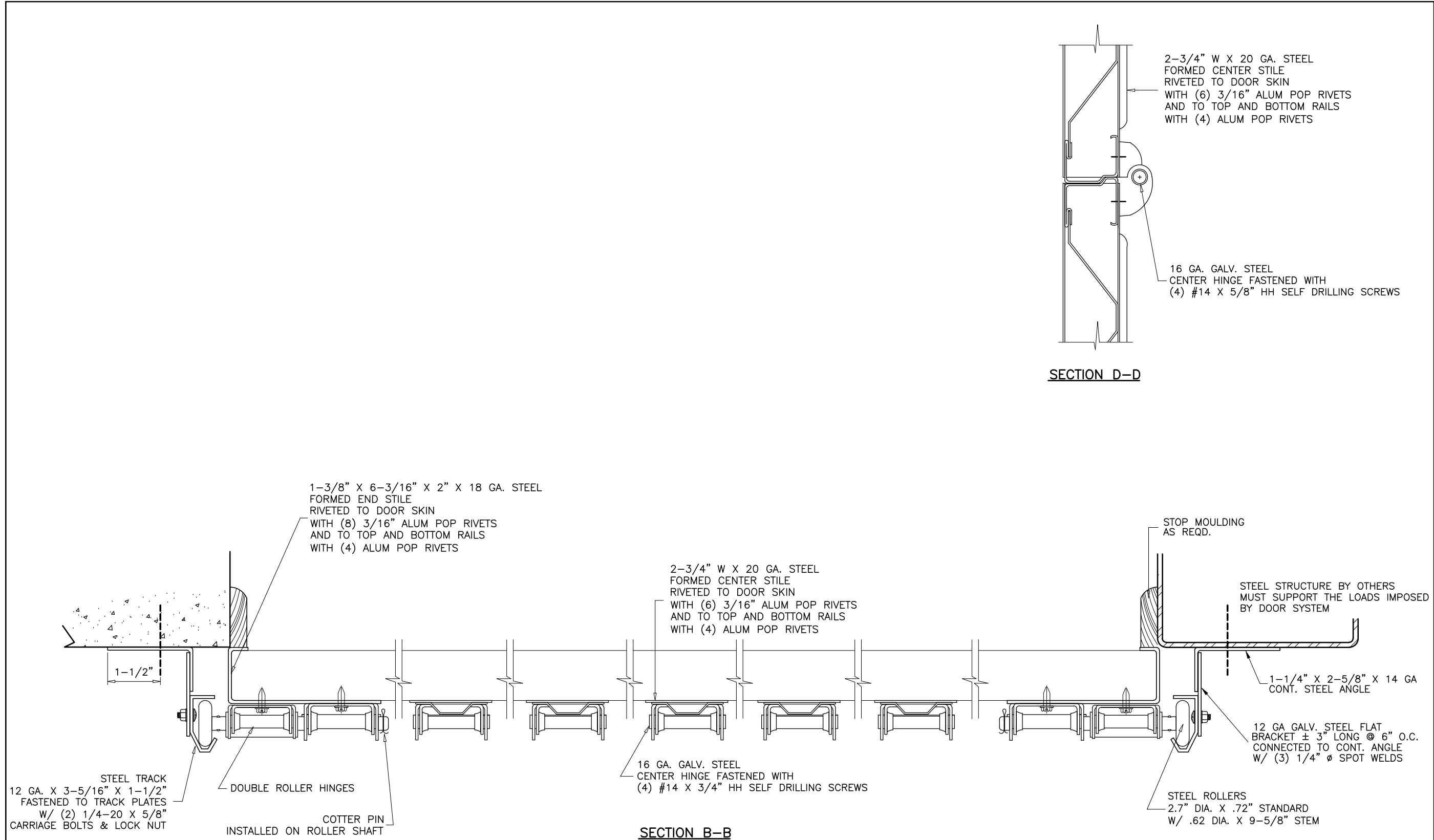
SECTION B-B
