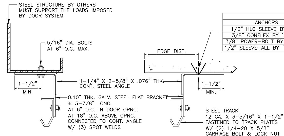
TRACK INSTALLATION
