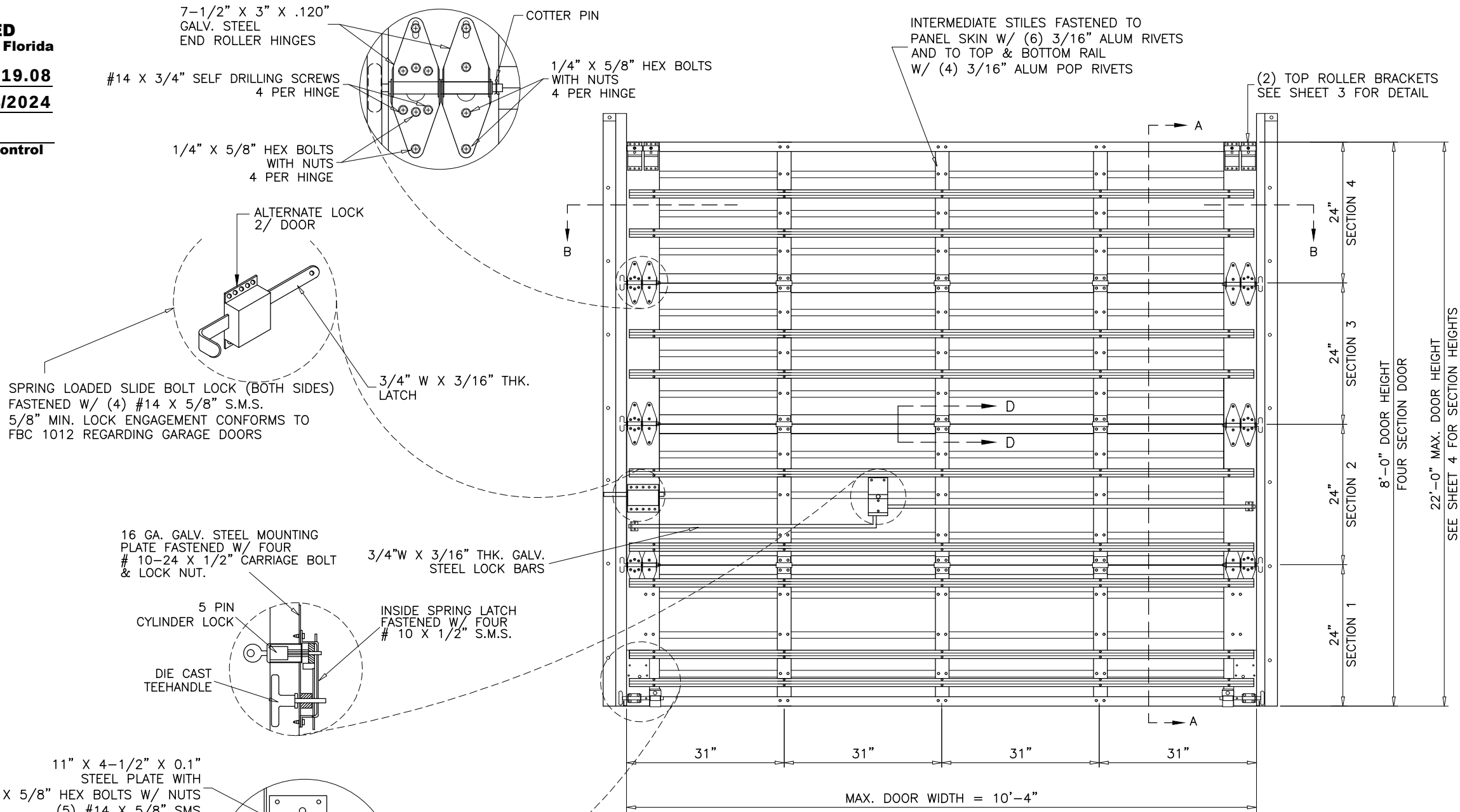
INSIDE ELEVATION
