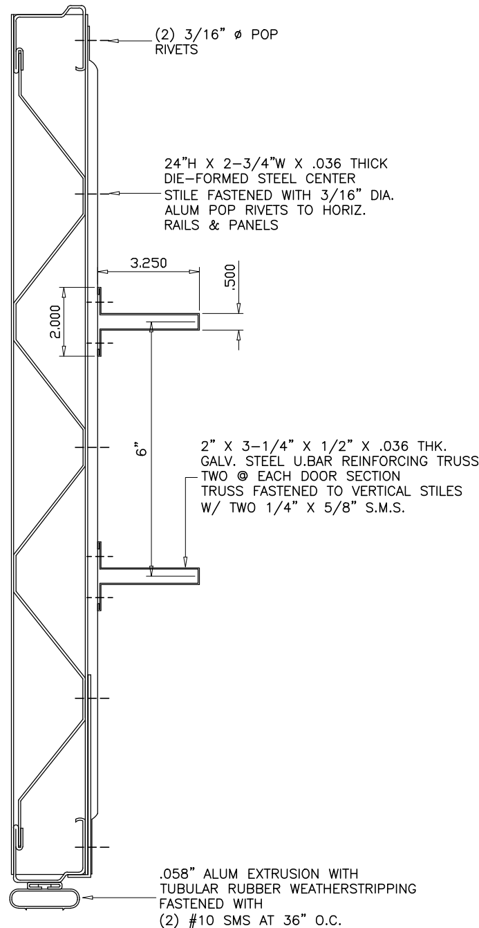
PANEL SECTION REINFORCEMENT
