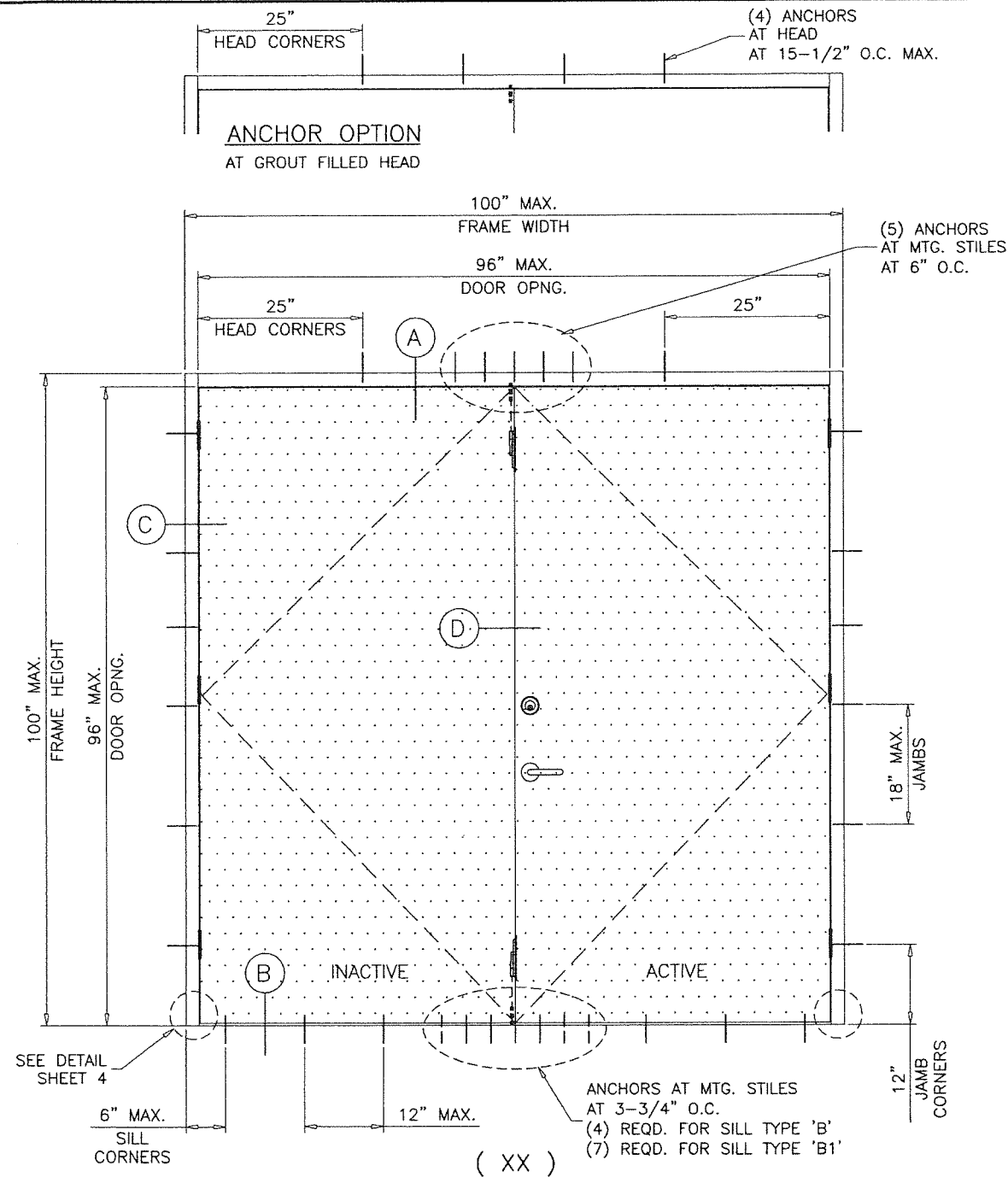
TYPICAL ELEVATIONS OPTION 1
