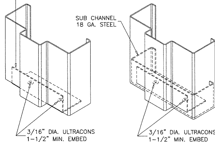
BOTTOM CORNER ANCHORS DETAIL
