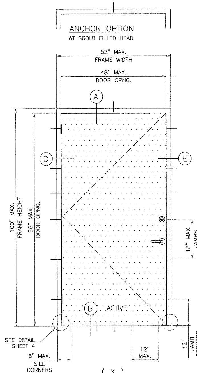
ANCHOR OPTION AT GROUT FILLED JAMBS
