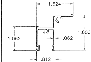
SASH BOTTOM RAIL C-3006 6063-T6
