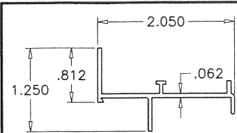
FRAME HEAD C-3001 6063-T6
