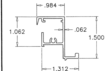
SASH TOP RAIL C-3005 6063-T6
