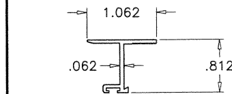
SASH SIDE RAIL C-3007 6063-T5
