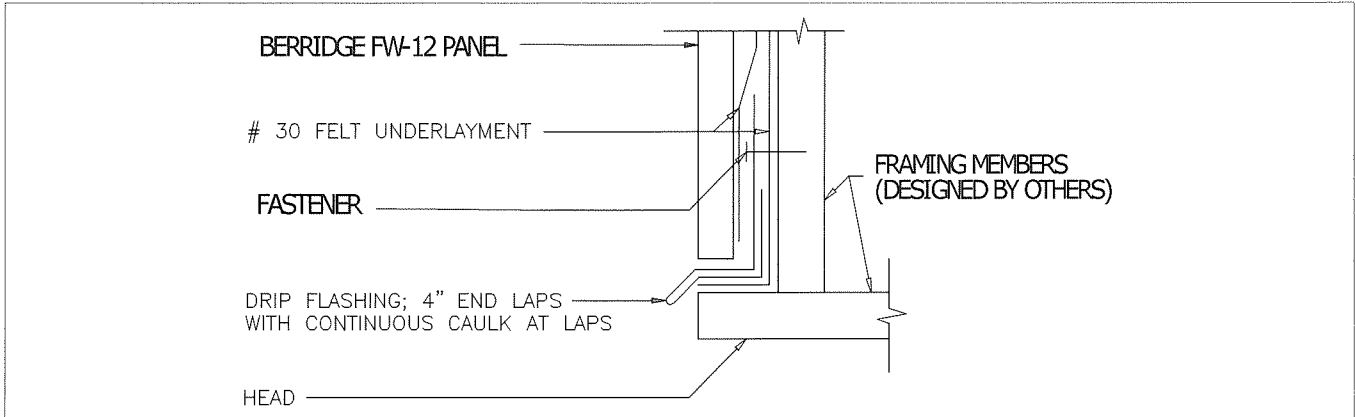
TYPICAL HEADER DETAIL
