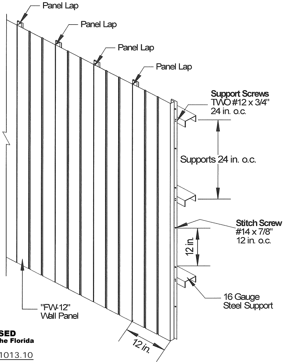
TYPICAL ELEVATION VIEW OUTSIDE OF WALL ASSEMBLY
