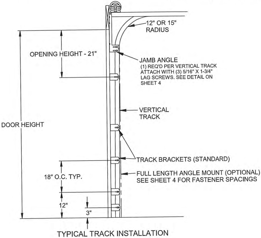
TYPICAL TRACK INSTALLATION
