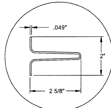
STEEL U-BAR DETAIL 18 GA. (.049" MIN) GALVANIZED HIGH TENSILE STEEL 80 KSI MINIMUM YIELD
