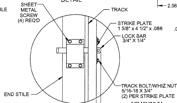
INTERIOR LOCK DETAIL
