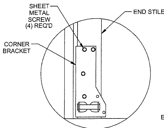
CORNER BRACKET DETAIL
