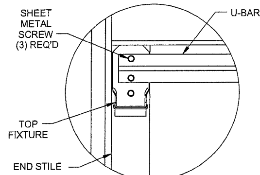
TOP FIXTURE / U-BAR DETAIL
