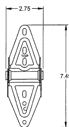
CENTER HINGE .045 GALV. STEEL
