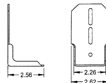
TOP FIXTURE .086 GALV. STEEL
