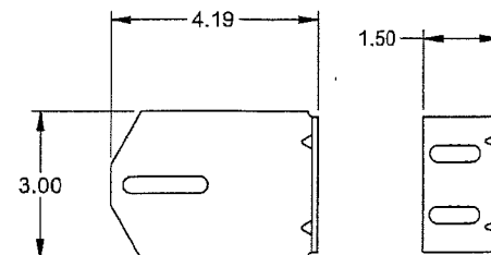
4" TRACK BRACKET .116 GALV. STEEL
