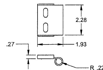
ROLLER CARRIER .086 GALV. STEEL ATTACHED TO TOP FIXTURE WITH (2) TRACK BOLTS AND WHIZ NUTS
