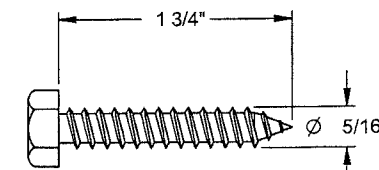
HEX HEAD LAG SCREW
