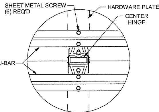
CENTER HINGE / U-BAR DETAIL
