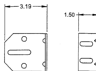
3" TRACK BRACKET .116 GALV. STEEL
