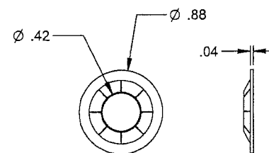
RETAINING NUT
