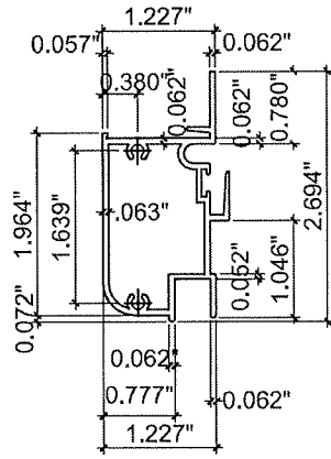
02 FIXED MEETING RAIL 6063-T6
