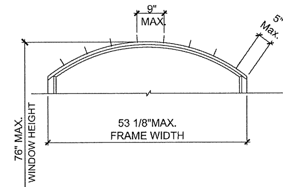
EYEBROW OPTION (FOR ORIAL OR EQUAL SASH)
