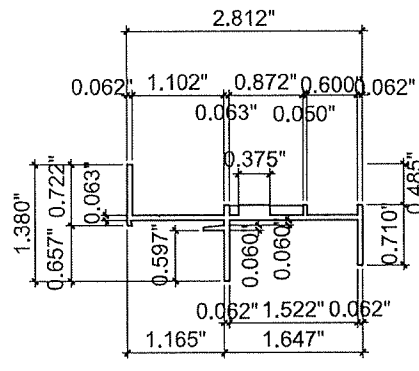
06 FRAME HEAD 6063-T6
