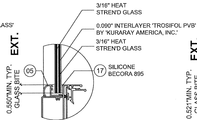
GLASS TYPE "B"
