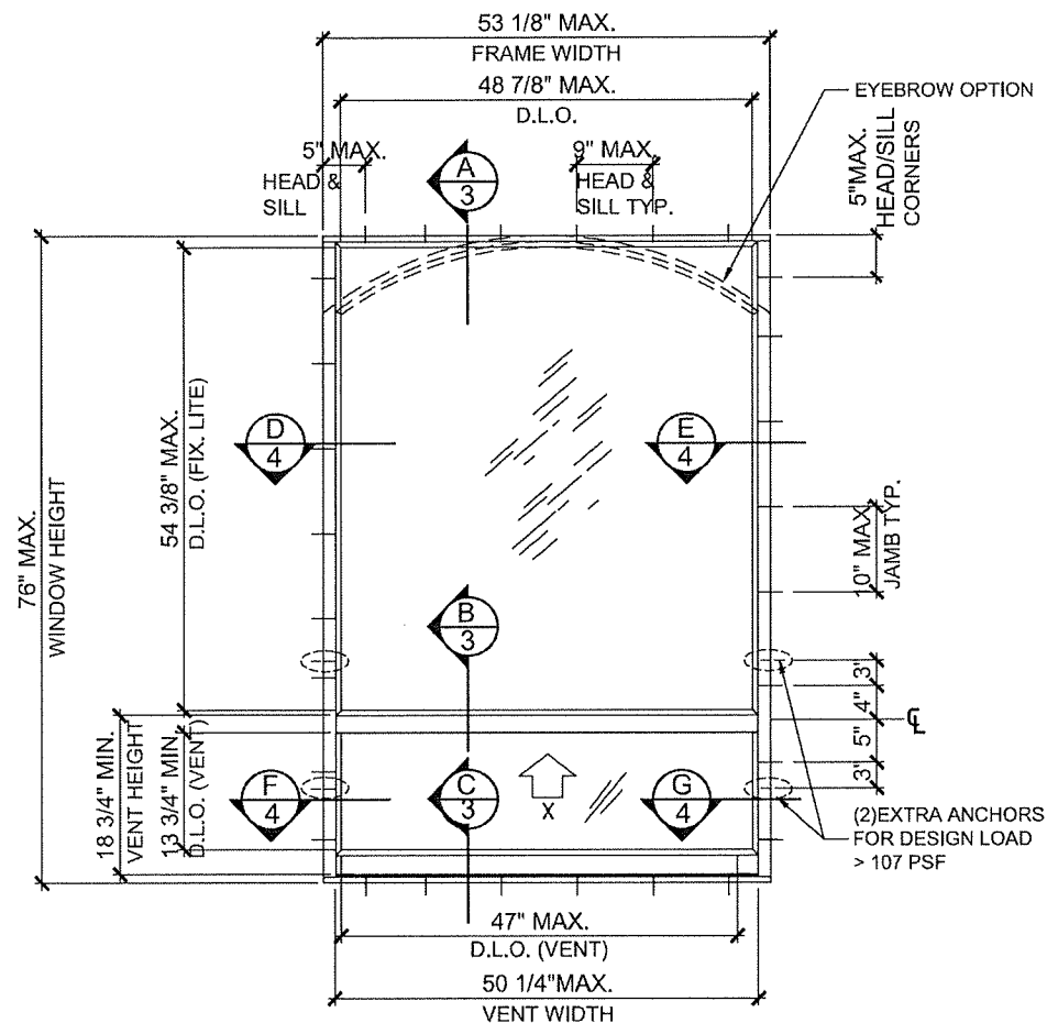
TYPICAL ELEVATION
