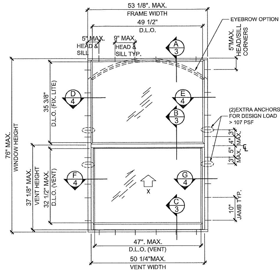
TYPICAL ELEVATION
