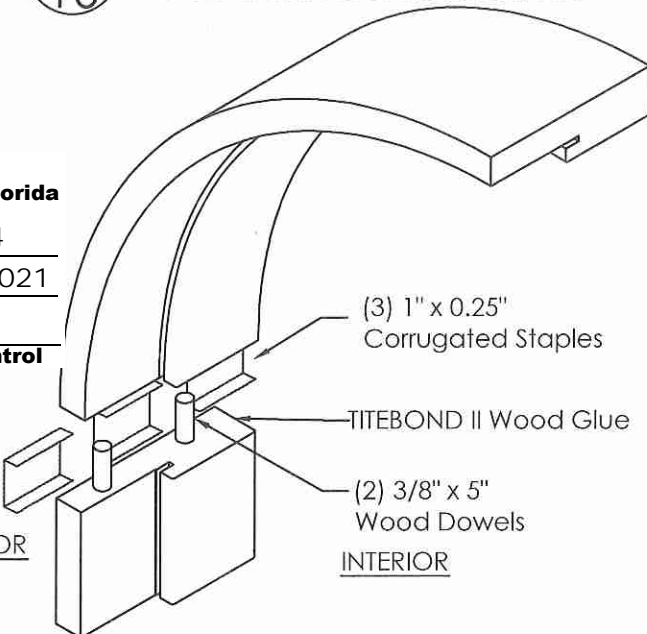
N 10 CORNER SECTION CURVED PANEL TOP ASSEMBLY, TYP.
