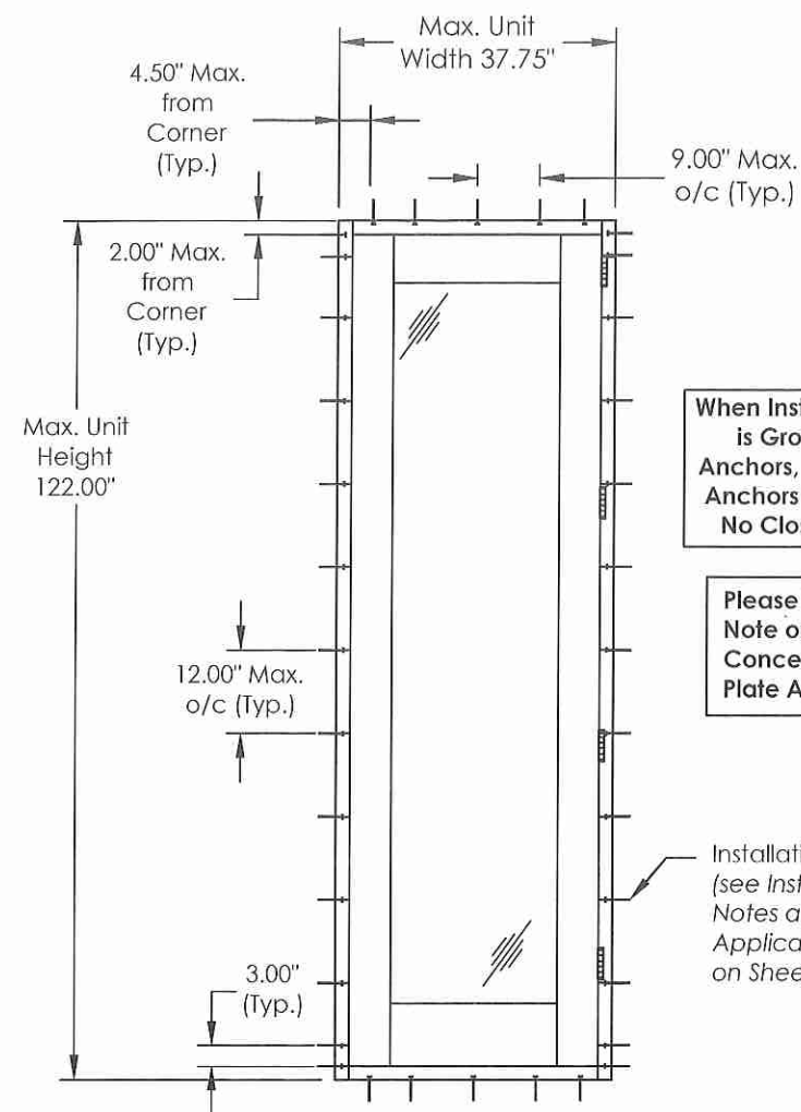
ANCHOR LAYOUT
