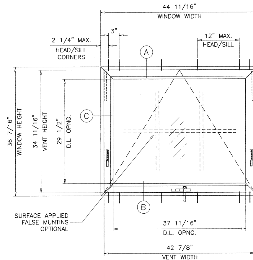
TYPICAL ELEVATION
