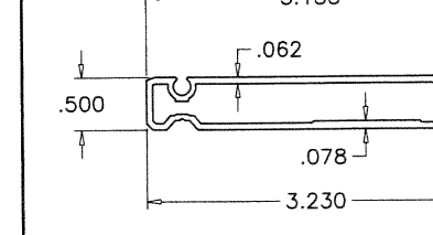
②⑧ FLUSH FRAME ADAPTER
