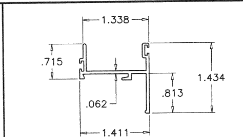
⑨ VENT TOP/BOTTOM RAIL
