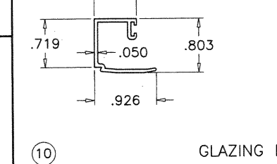
①⑩ GLAZING BEADS
