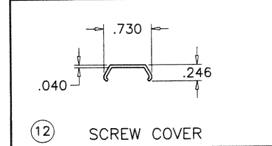
①② SCREW COVER
