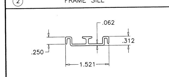
③ SILL TRACK
