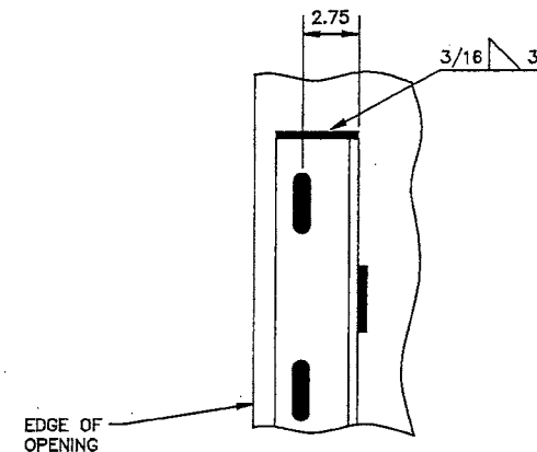
FRONT VIEW OF WALL ANGLE
