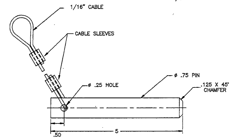
DETAIL "F"
