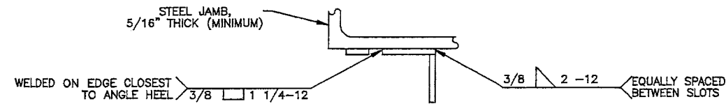
TOP VIEW
