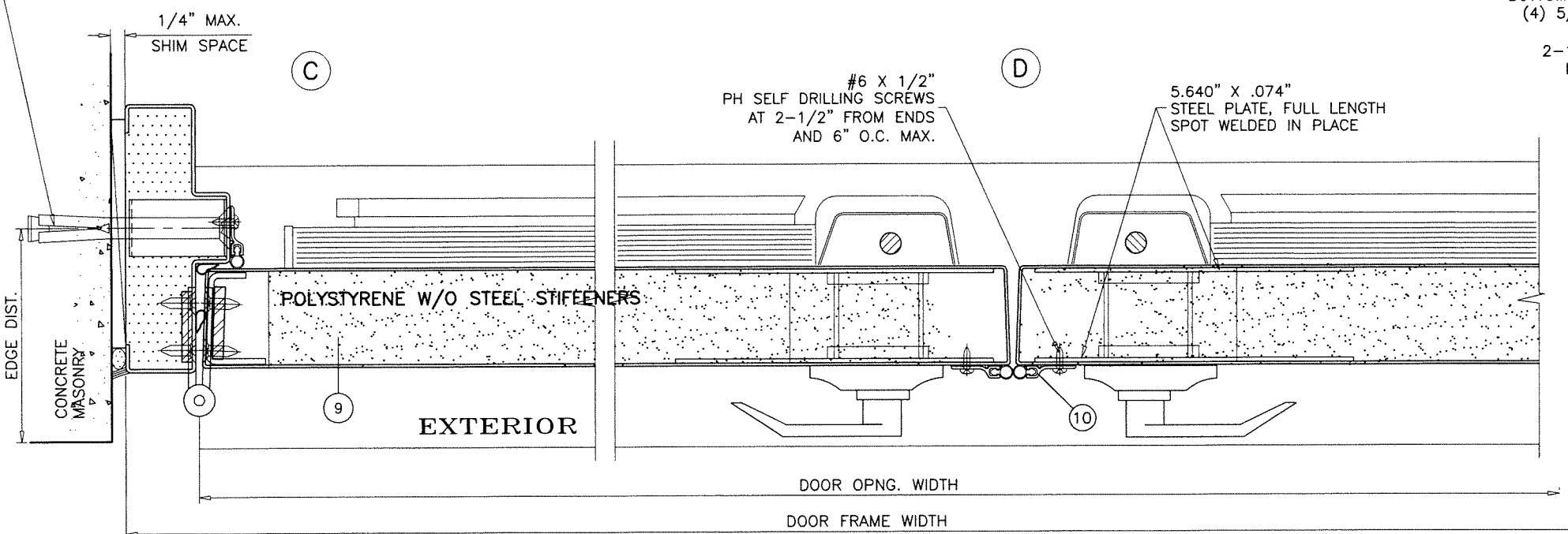
LOCK OPTION #4 (PHG 9700 PANIC W/ SURFACE VERTICAL RODS)
