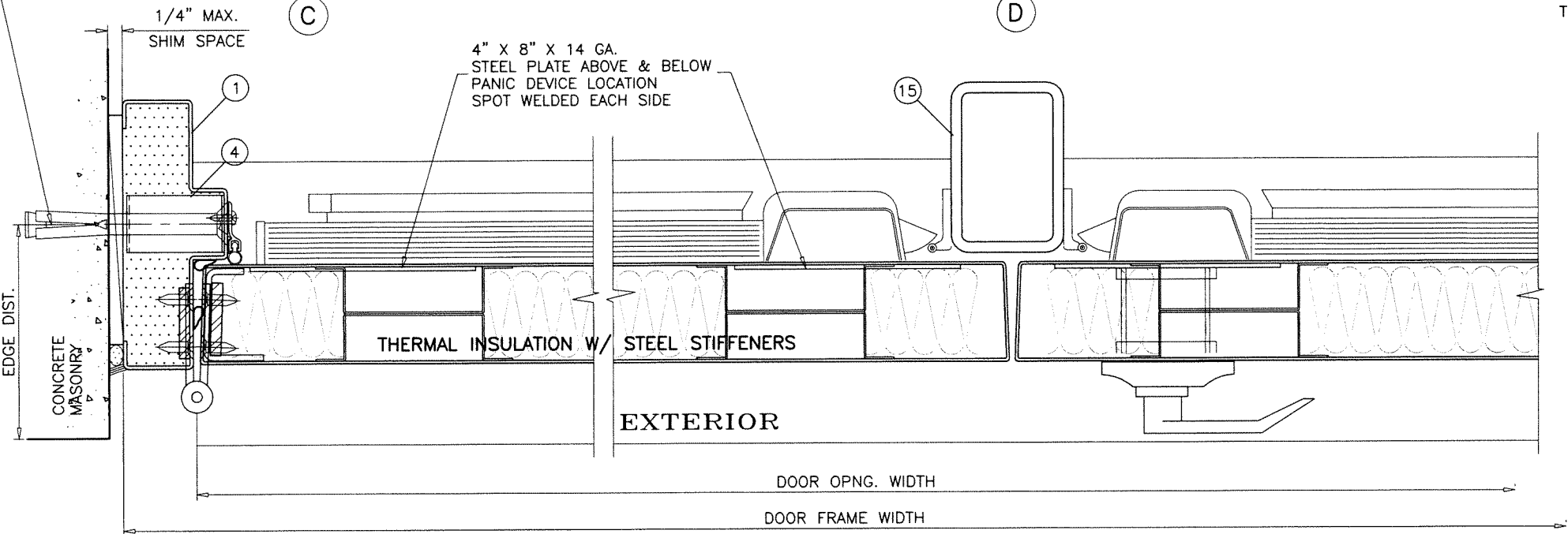
LOCK OPTION #3 (PHG 9500 RIM PANIC W/ PHG 9000 SERIES MULLION)
