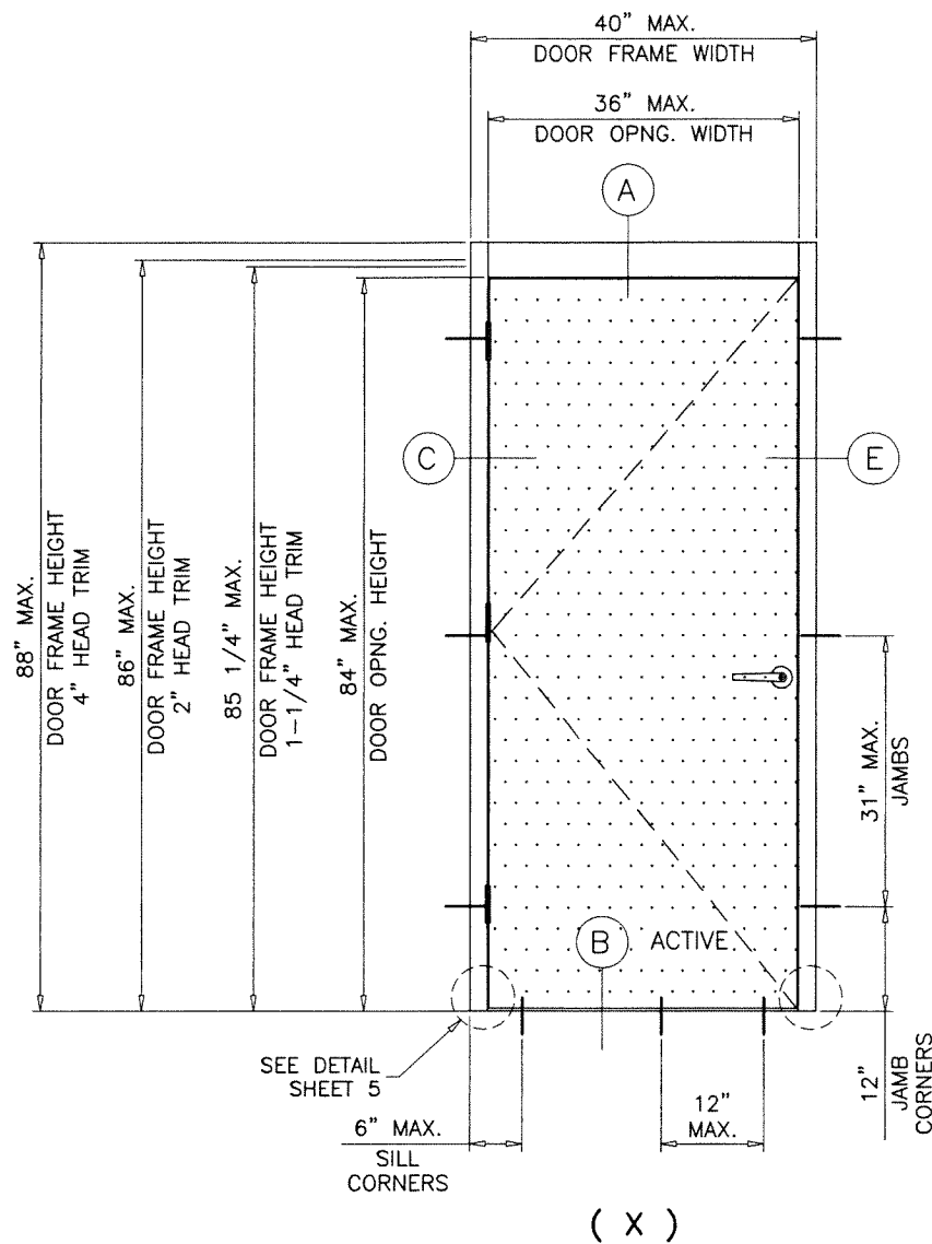
TYPICAL ELEVATIONS
