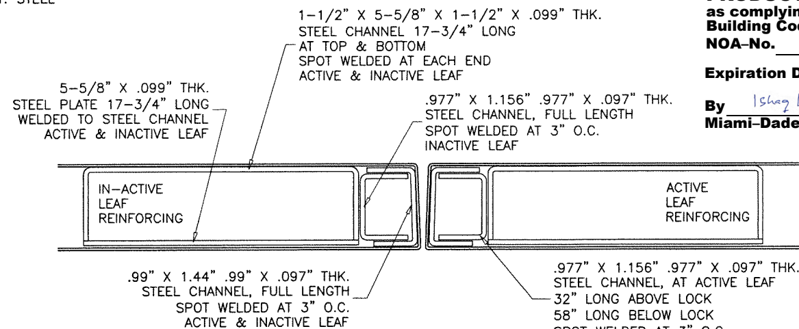
LOCK STILES REINFORCING
