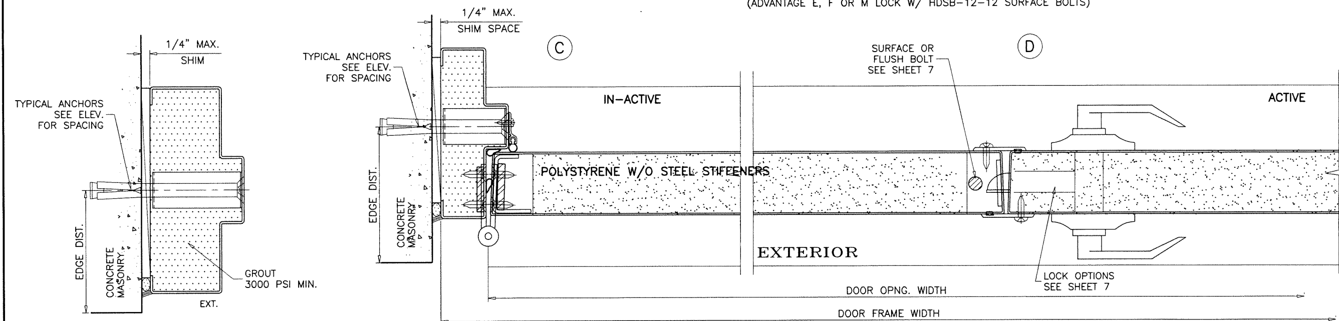
LOCK OPTION #1 & #2 (ADVANTAGE E, F OR M LOCK W/ HDSB-12-12 SURFACE BOLTS)
