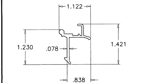
M12 SPRING LOADED LATCH
