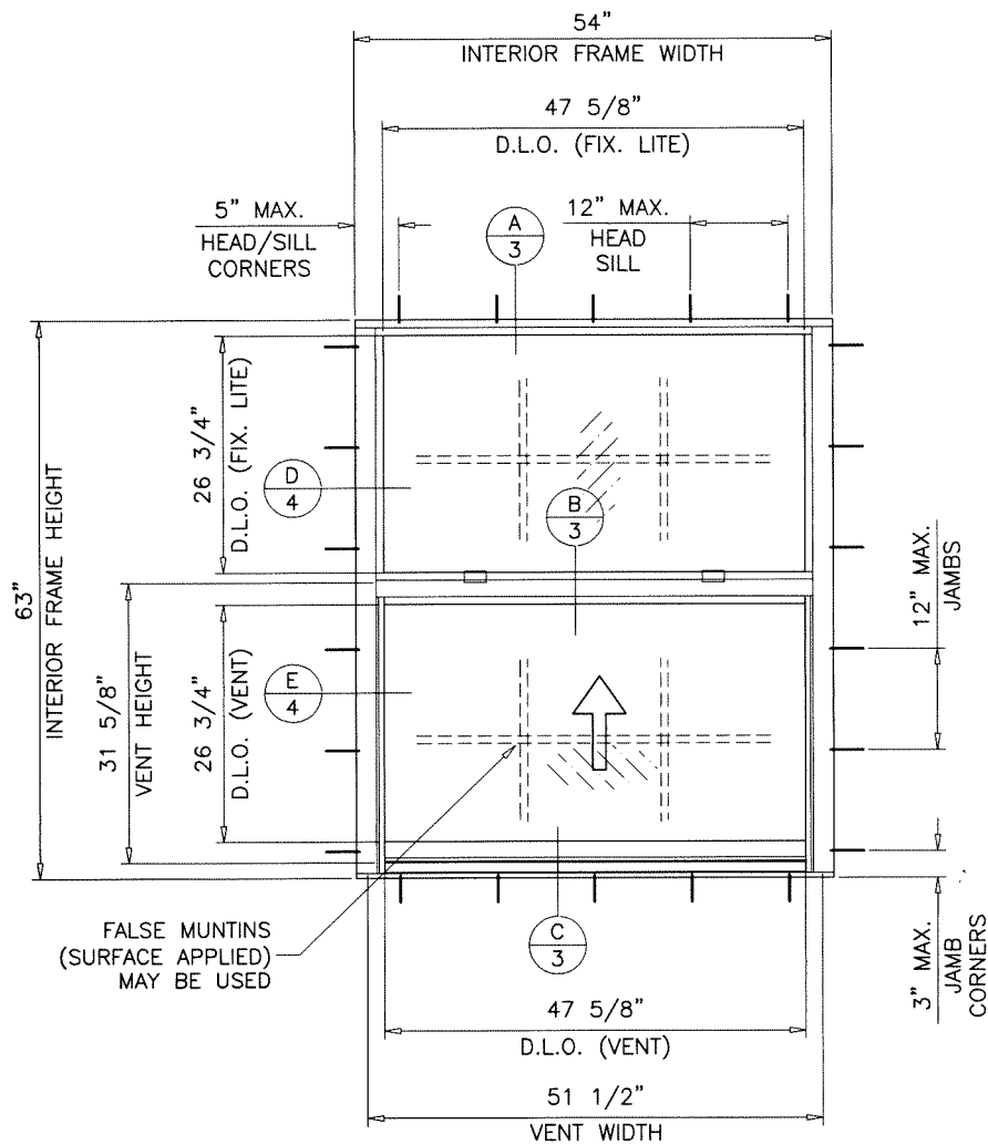
TYPICAL ELEVATION
