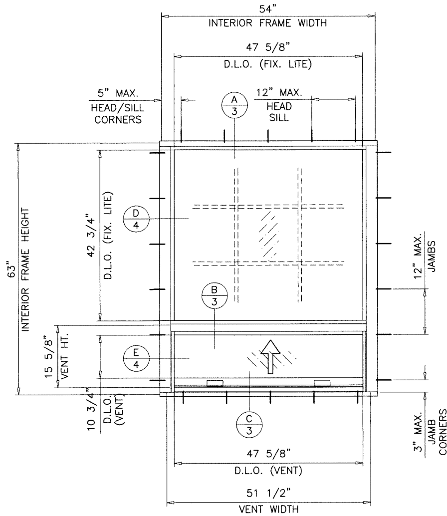
TYPICAL ELEVATION
