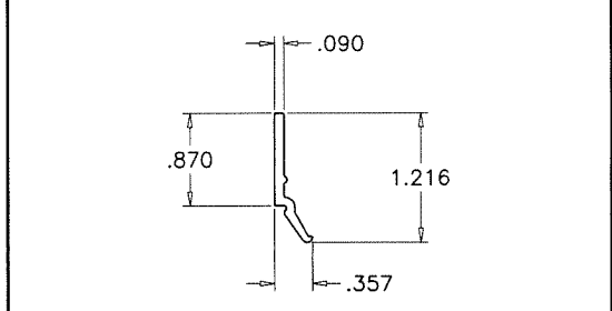
E02 GLAZING BEAD
