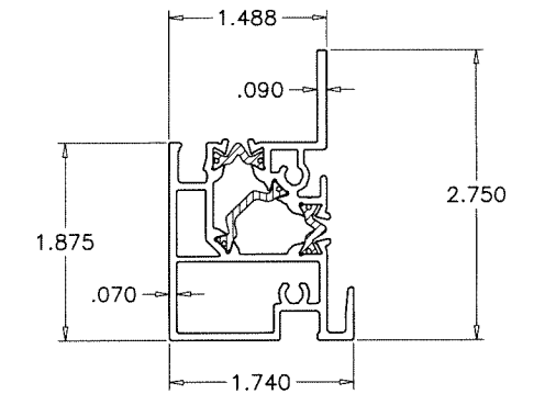
E09 FIX. MEETING RAIL
