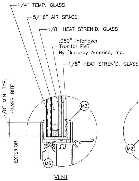
GLAZING DETAILS
