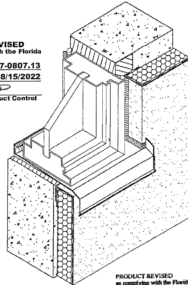
WINDOW OPENING
