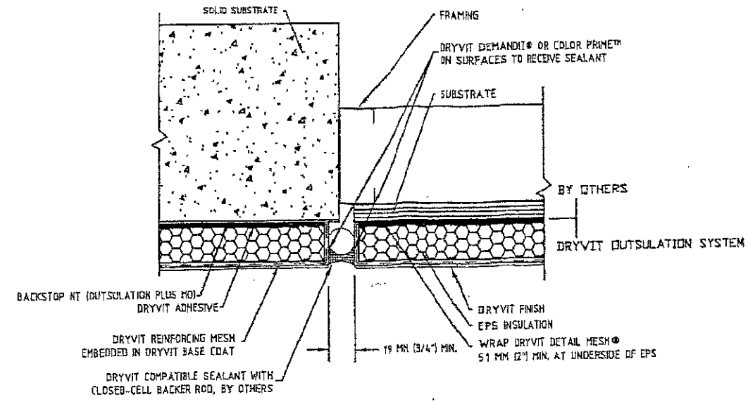
EXPANSION JOINT
