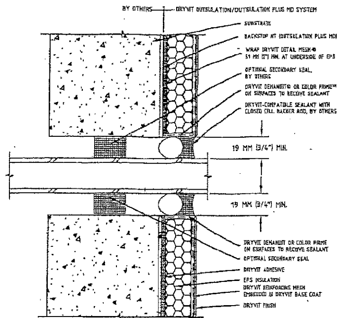
PENETRATIONS
