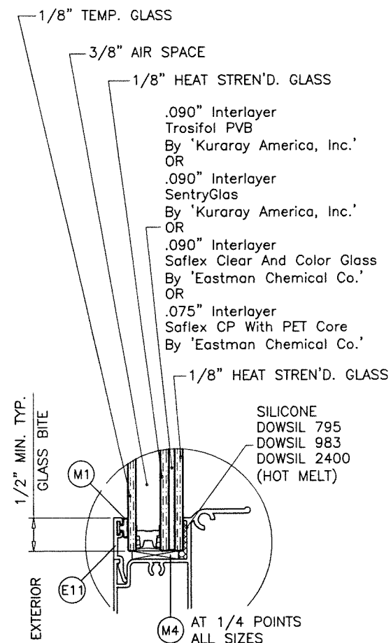
GLASS TYPE '1i' 7/8" OVERALL INSUL. LAM. GLASS
