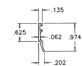
E11 GLAZING BEADS
