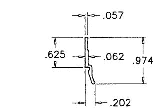
E11A GLAZING BEADS
