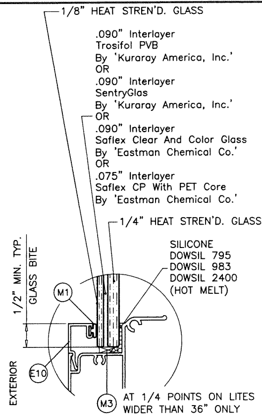
GLASS TYPE '2' 7/16" OVERALL LAM. GLASS
