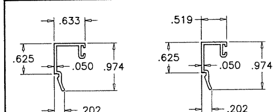
E9 GLAZING BEADS
