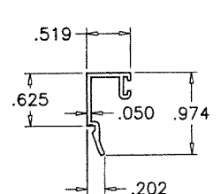
E9 GLAZING BEADS
