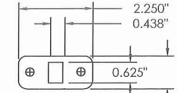
SHOOTBOLT STRIKE PLATE Face View
