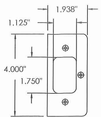
DEADBOLT STRIKE PLATE Face View
