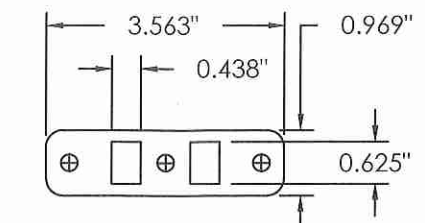
DOUBLE SHOOTBOLT STRIKE PLATE Face View
