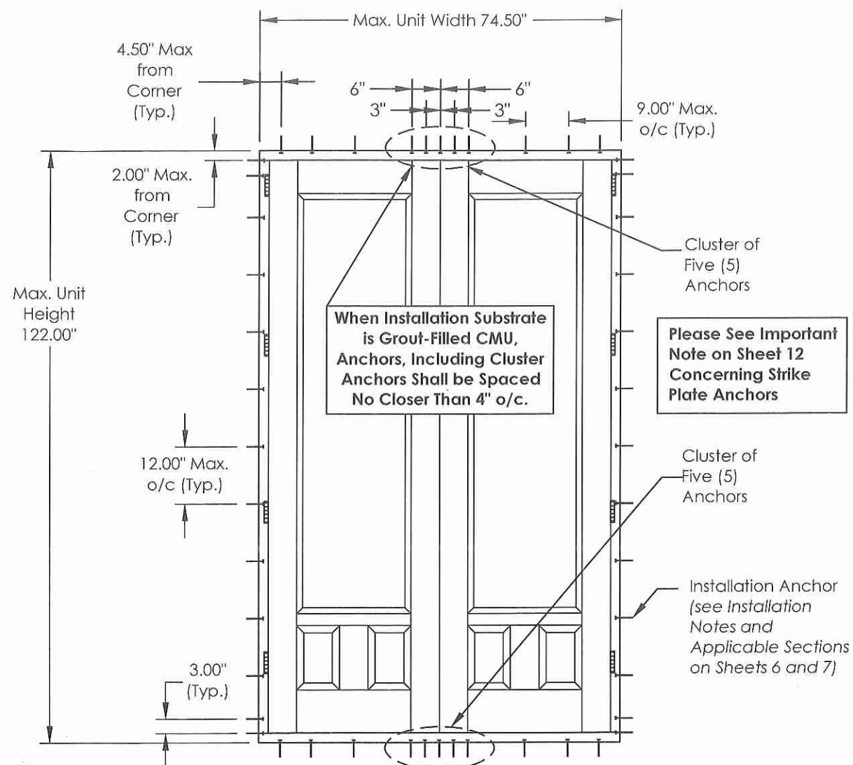
ANCHOR LAYOUT
