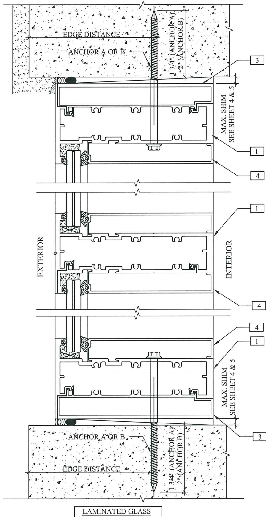
DETAIL A
