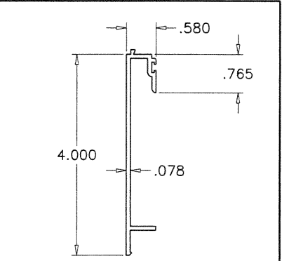
②.1 TOP/BOTTOM RAIL (TRIMMED) SURFACE APPLIED CHAIR RAIL
