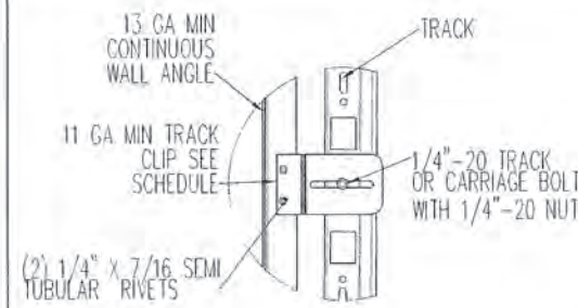
TYPICAL TRACK CLIP RIVETING DETAIL
