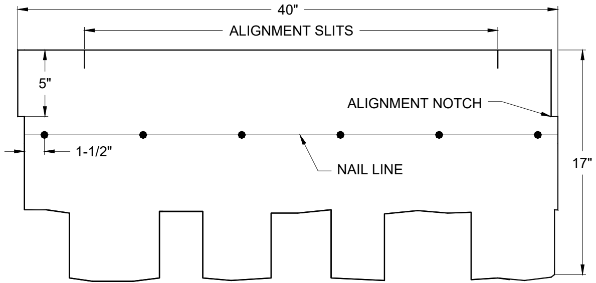
TOP OF SHINGLE
