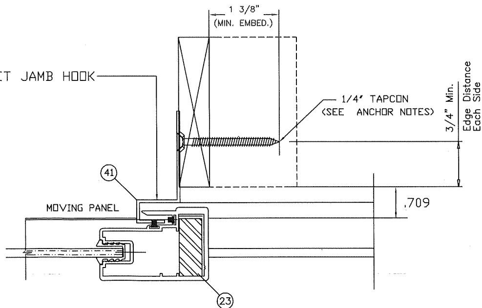
POCKET DOOR JAMB ANCHOR DETAIL
