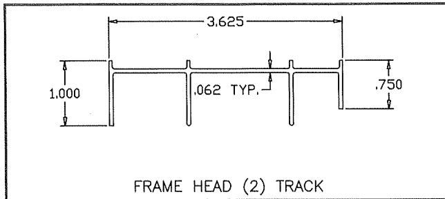
FRAME HEAD (2) TRACK
