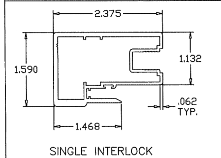
SINGLE INTERLOCK
