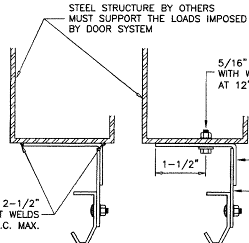
REVERSE TRACK TO STEEL
