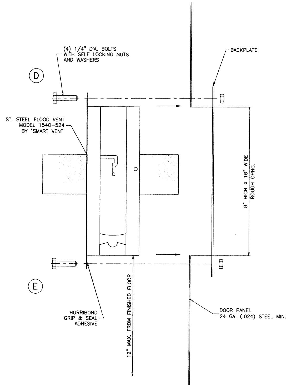
FLOOD VENT DETAIL AUTOMATIC NON-POWERED ACTIVATION & OPERATION
