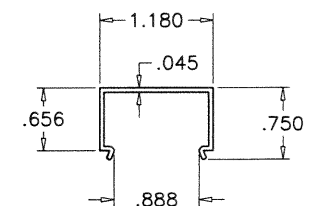
COVER CHANNEL GOP-8
