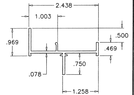
FRAME HEAD/SILL GOP-10
