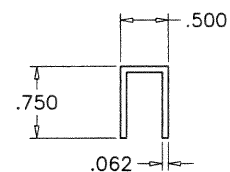
GLAZING STOP GOP-9
