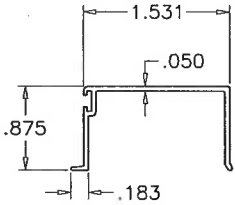
2 GLAZING BEAD
