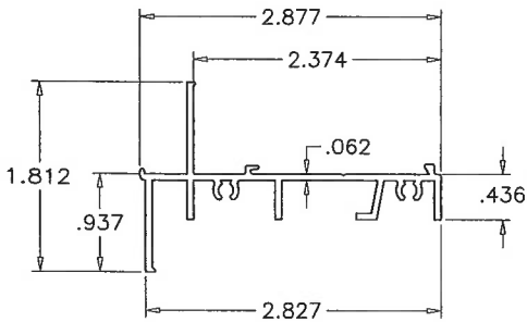
1 FRAME HEAD/SILL/JAMB
