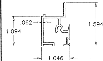
4 MEETING RAIL 6063-T6
