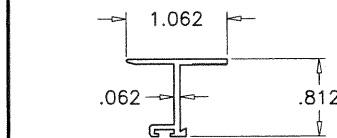
8 SASH SIDE RAIL 6063-T5
