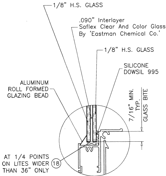
GLAZING DETAIL
