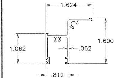
6 SASH BOTTOM RAIL 6063-T6
