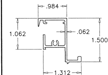
5 SASH TOP RAIL 6063-T6
