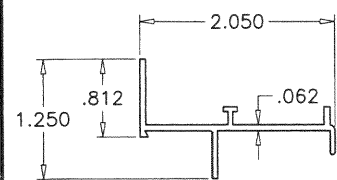
1 FRAME HEAD 6063-T6
