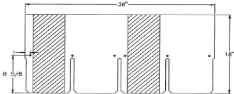
Detail B Overall Dimensions and Nailing Pattern
