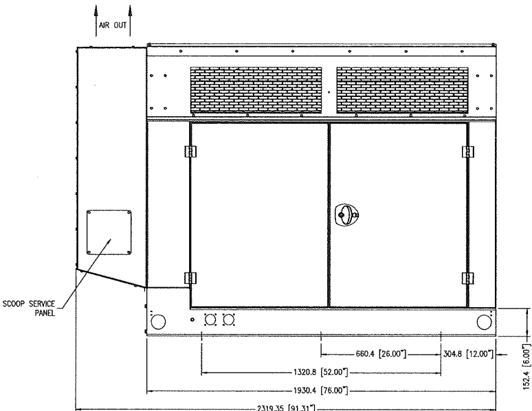
LEFT VIEW
