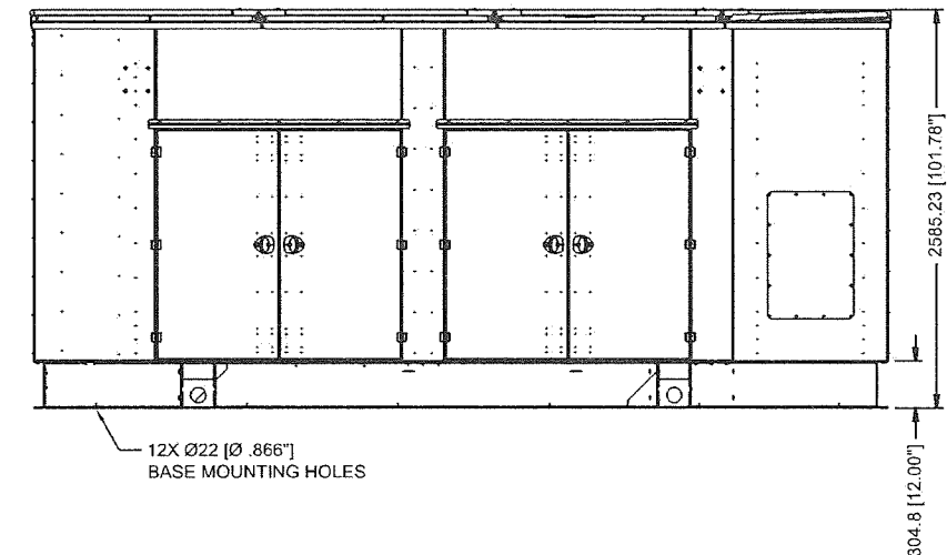
RIGHT VIEW
