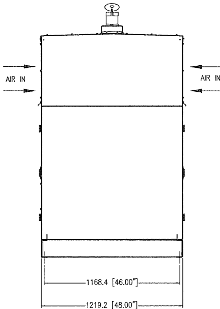
REAR VIEW
