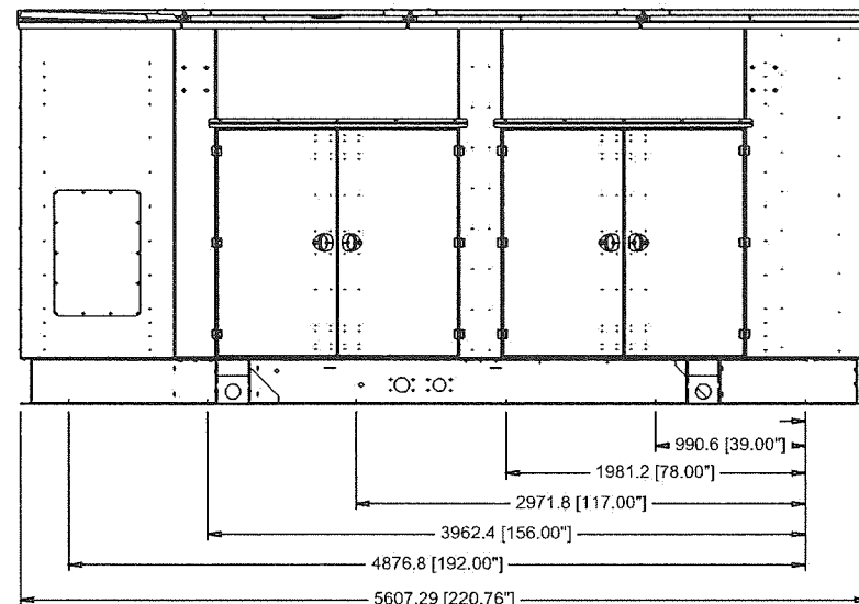
LEFT VIEW
