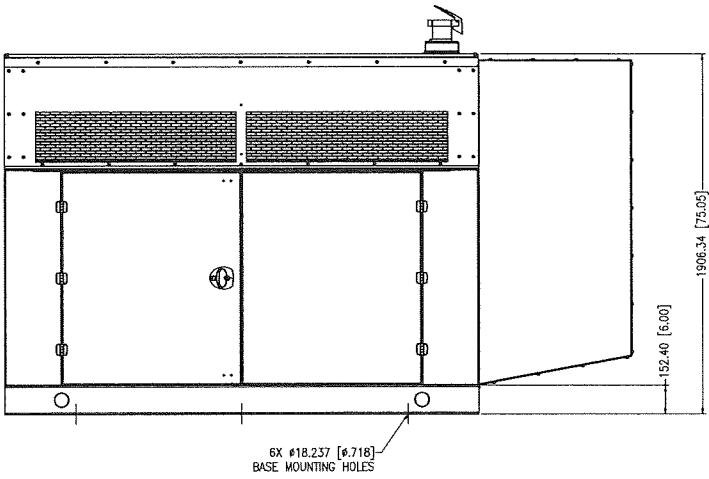
RIGHT VIEW
