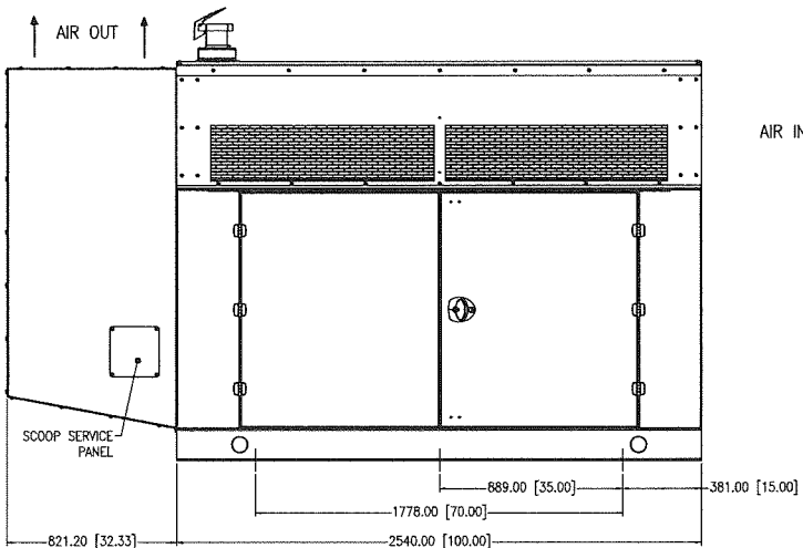
LEFT VIEW
