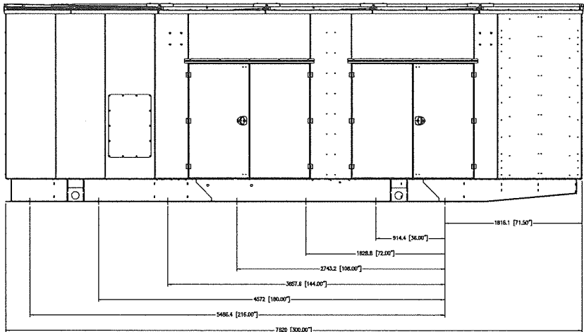
LEFT VIEW
