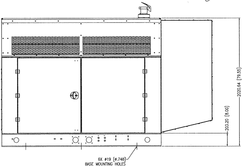
RIGHT VIEW
