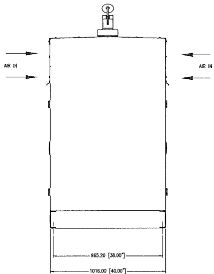
REAR VIEW
