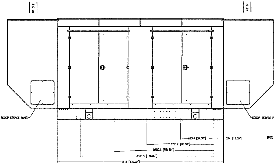
LEFT VIEW
