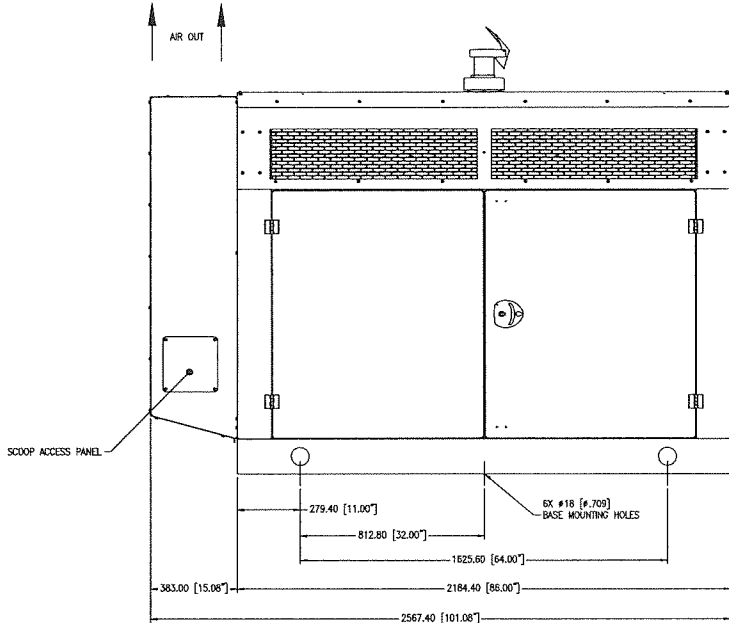
LEFT VIEW
