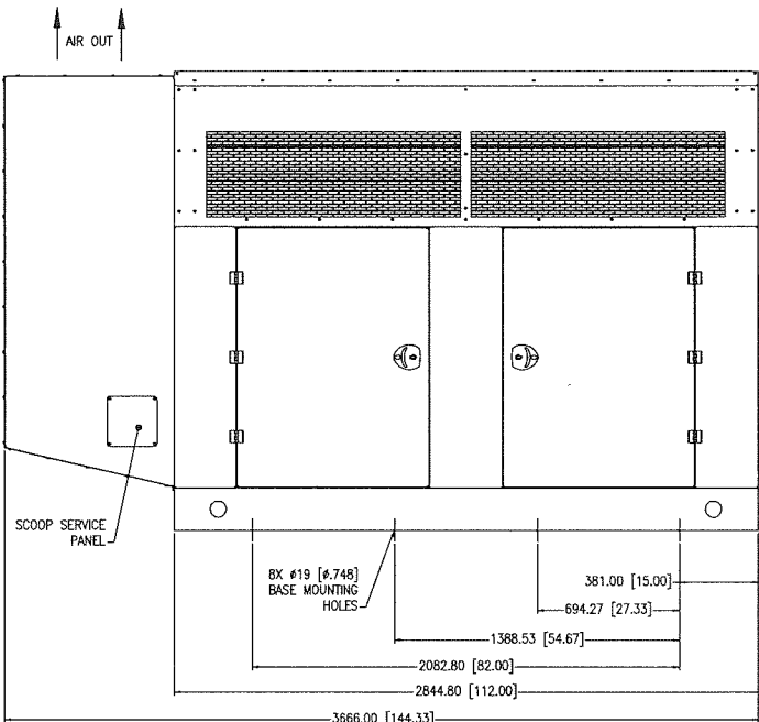
LEFT VIEW
