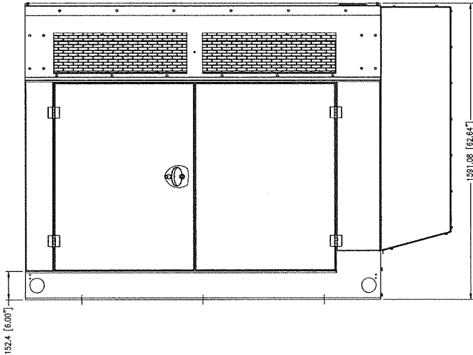
RIGHT VIEW
