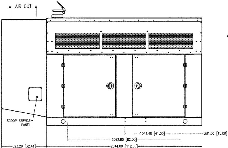
LEFT VIEW
