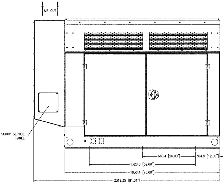
LEFT VIEW
