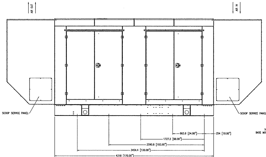
LEFT VIEW
