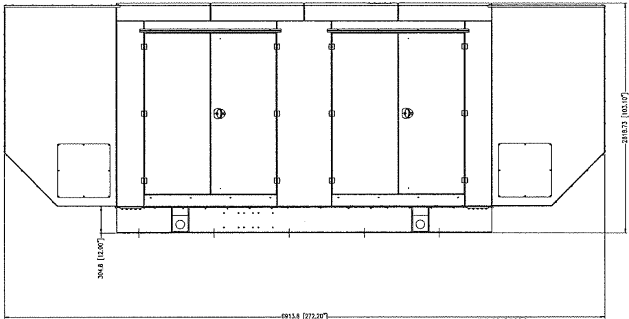
RIGHT VIEW
