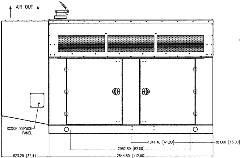
LEFT VIEW
