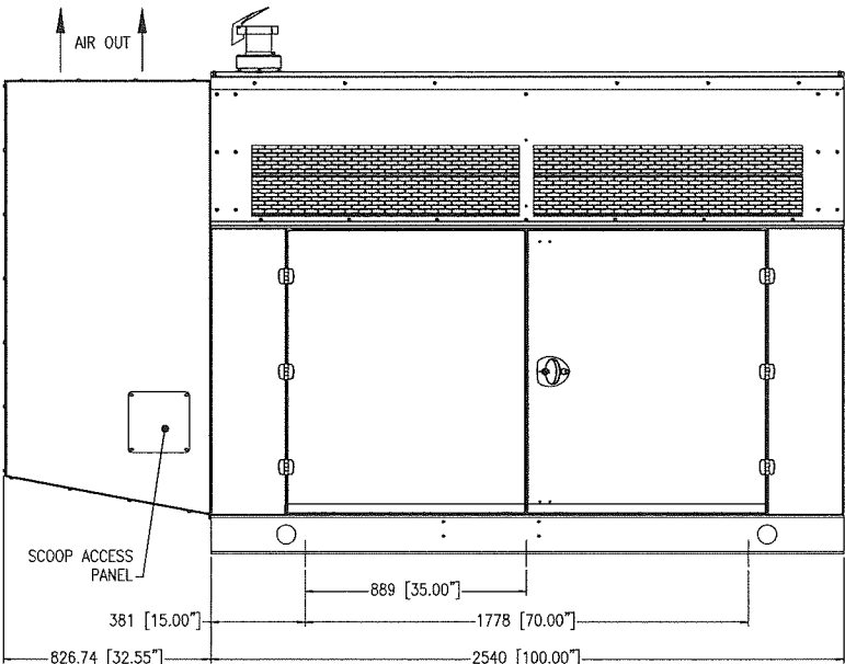
LEFT VIEW
