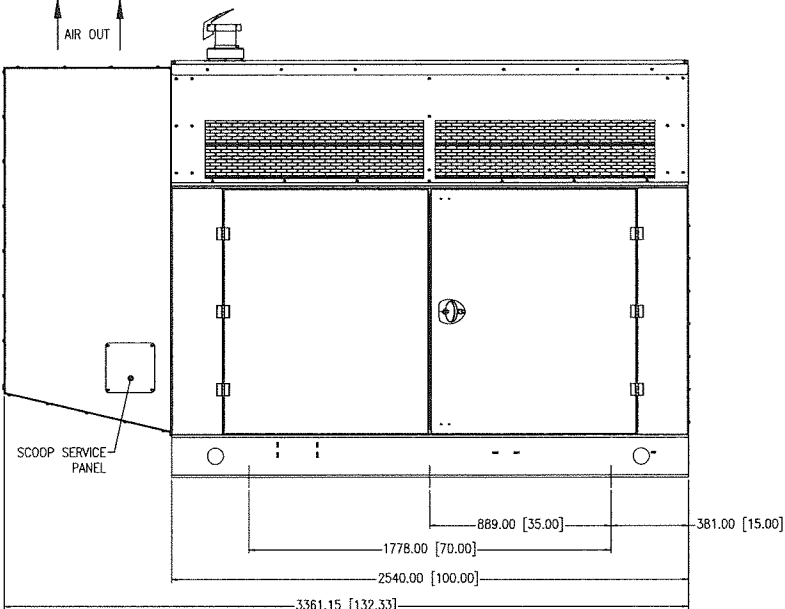
LEFT VIEW
