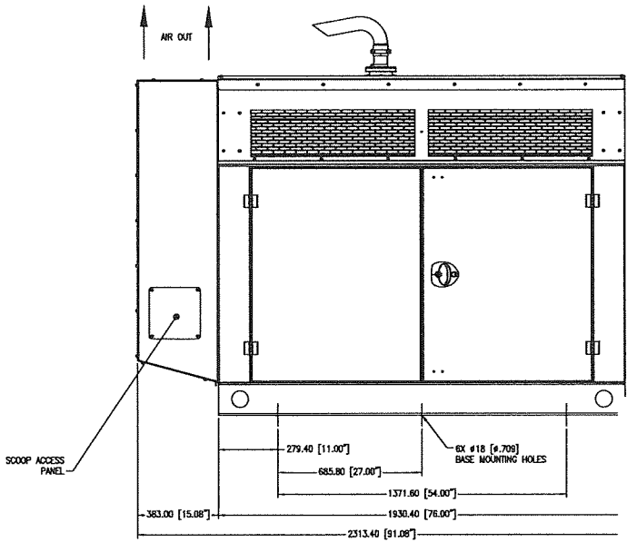
LEFT VIEW
