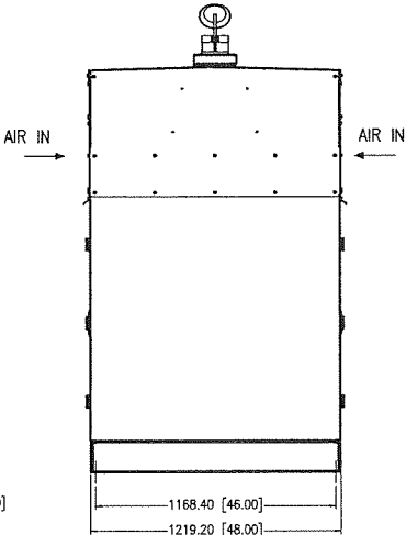
REAR VIEW
