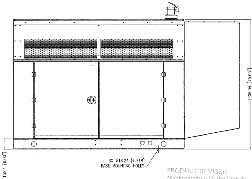
RIGHT VIEW
