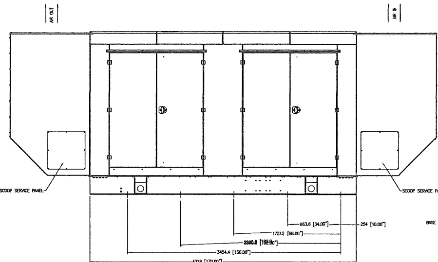
LEFT VIEW
